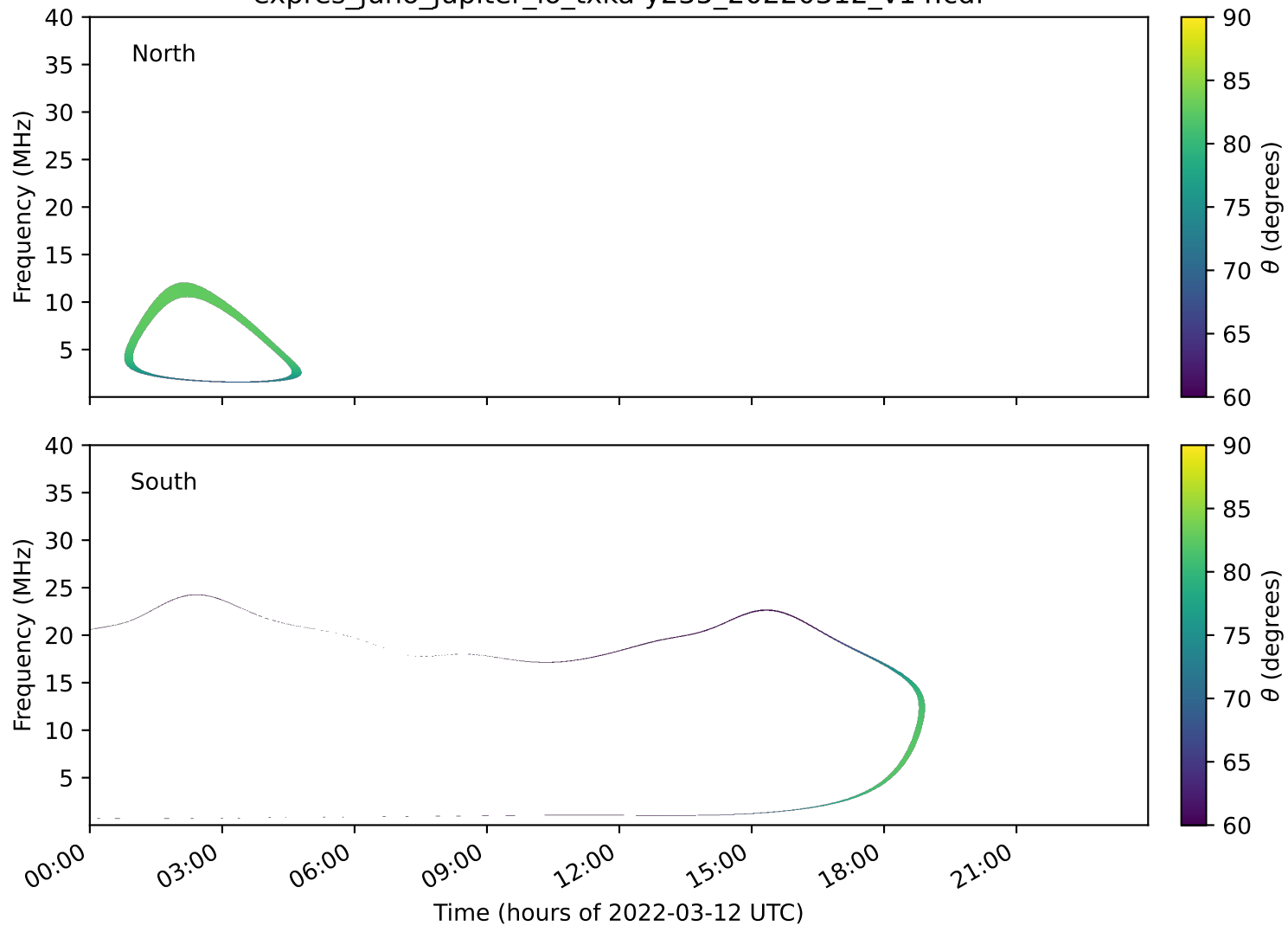
expres_juno_jupiter_io_txka-y235_20220312_v14.cdf
