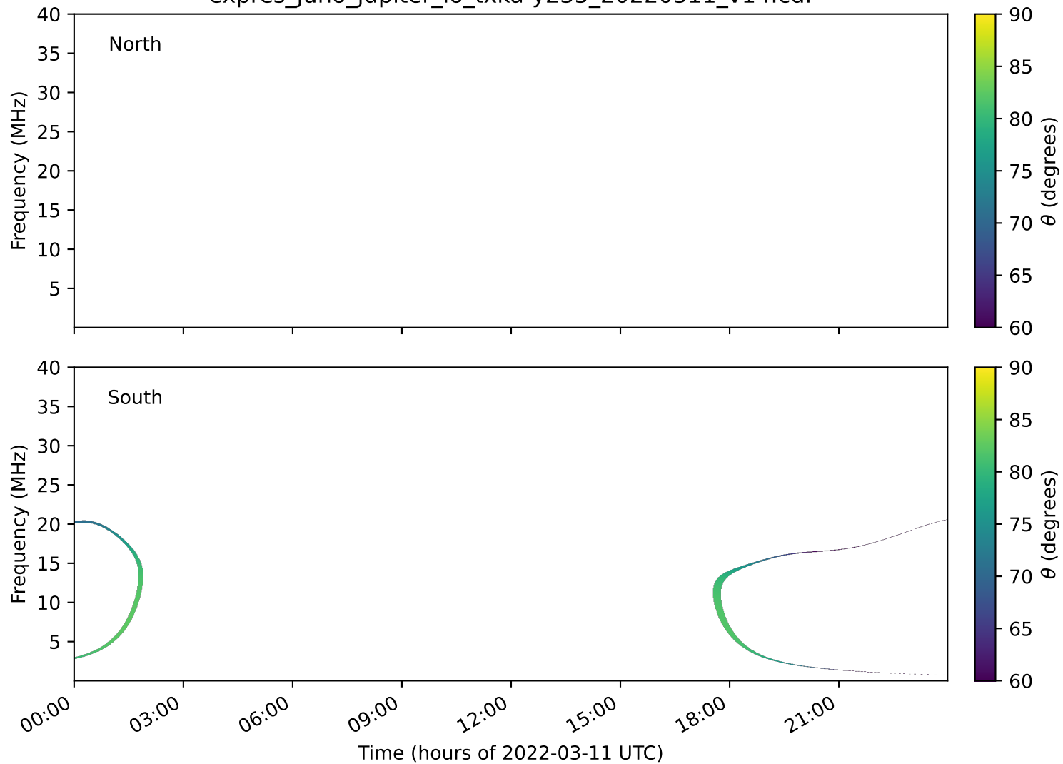
expres_juno_jupiter_io_txka-y235_20220311_v14.cdf
