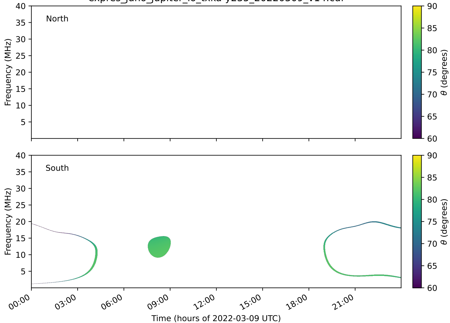
expres_juno_jupiter_io_txka-y235_20220309_v14.cdf
