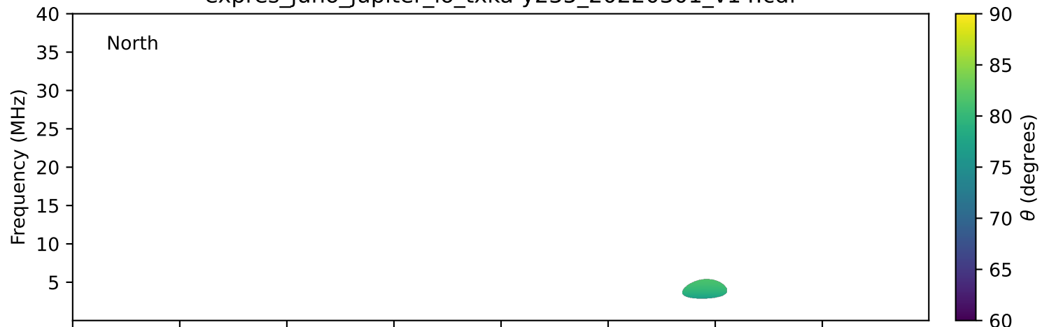
expres_juno_jupiter_io_txka-y235_20220301_v14.cdf
