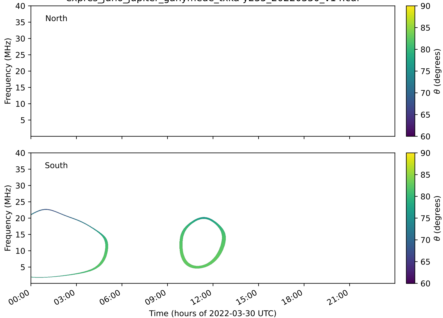
expres_juno_jupiter_ganymede_txka-y235_20220330_v14.cdf
