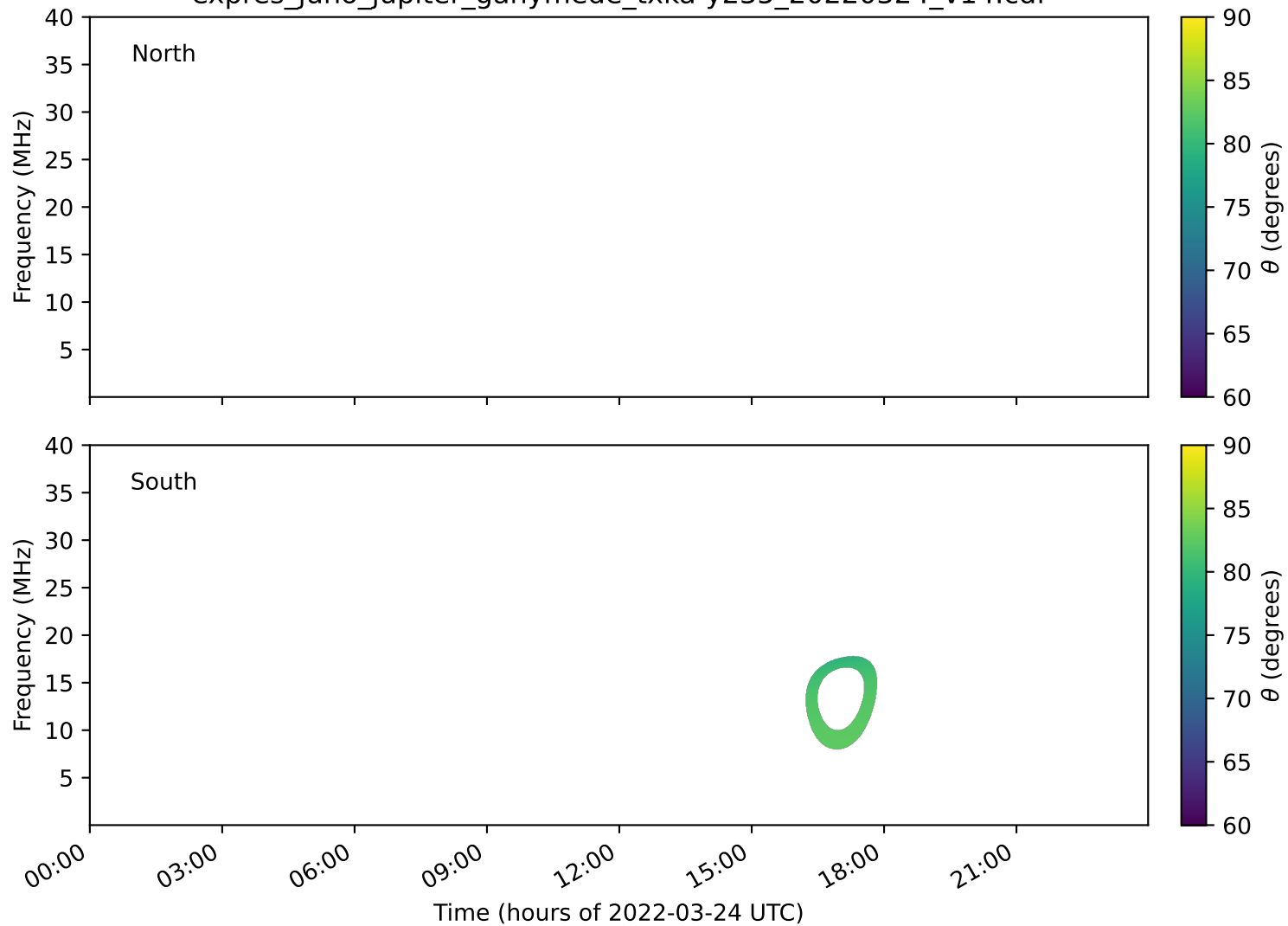
expres_juno_jupiter_ganymede_txka-y235_20220324_v14.cdf
