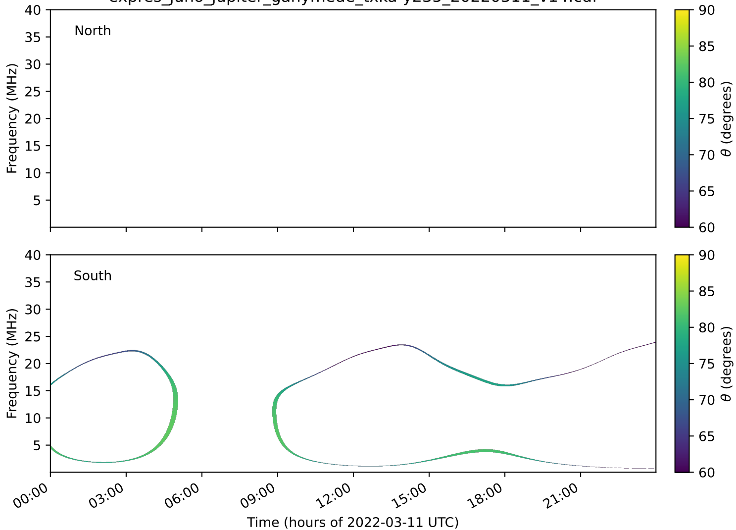
expres_juno_jupiter_ganymede_txka-y235_20220311_v14.cdf
