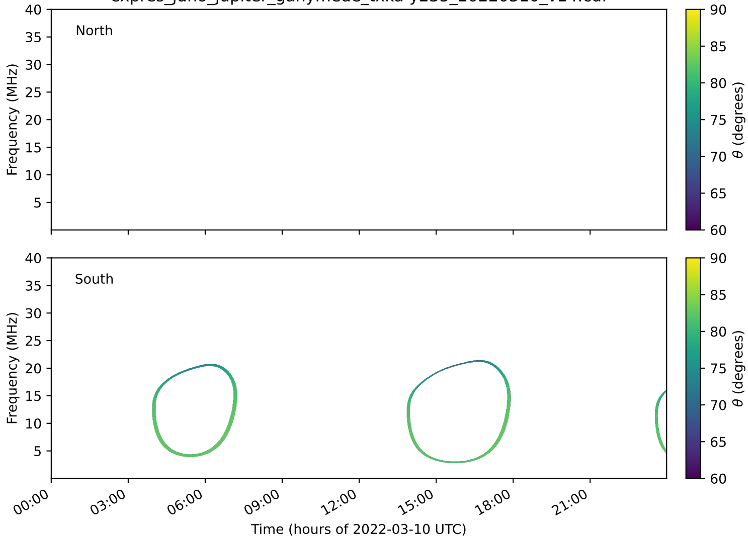
expres_juno_jupiter_ganymede_txka-y235_20220310_v14.cdf
