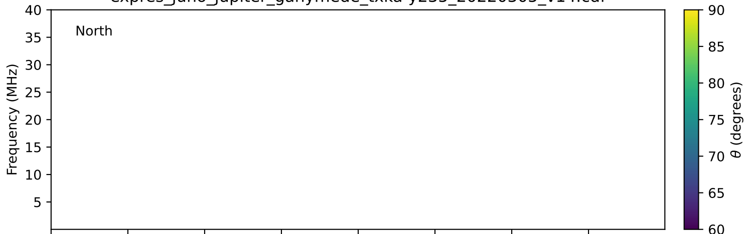
expres_juno_jupiter_ganymede_txka-y235_20220305_v14.cdf
