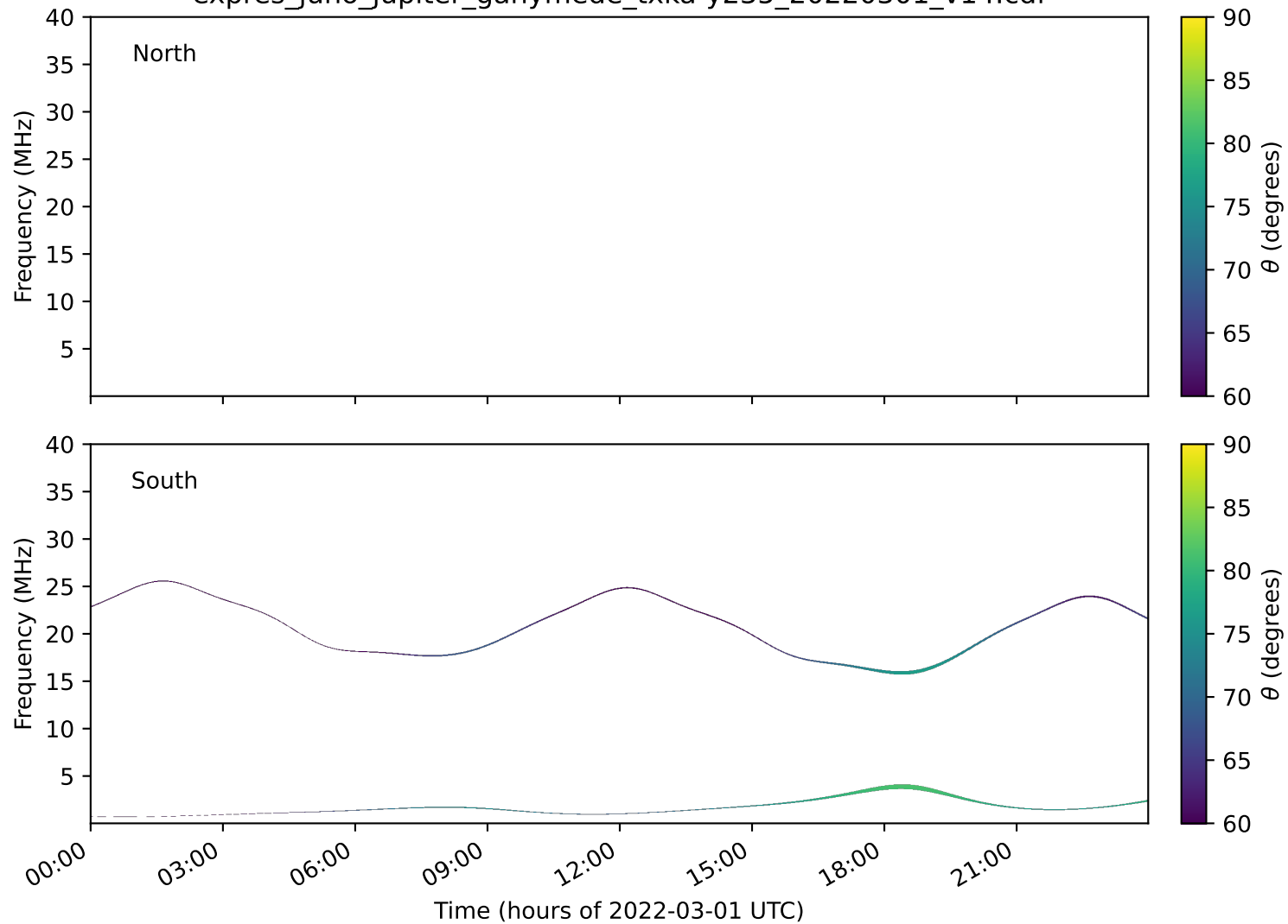
expres_juno_jupiter_ganymede_txka-y235_20220301_v14.cdf
