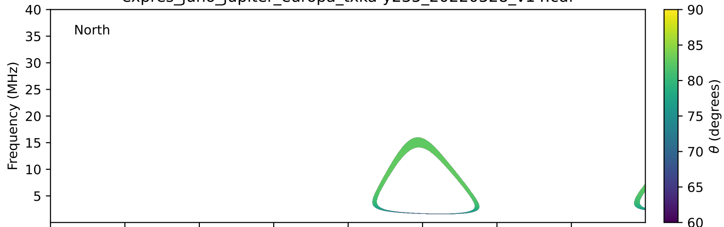
expres_juno_jupiter_europa_txka-y235_20220328_v14.cdf
