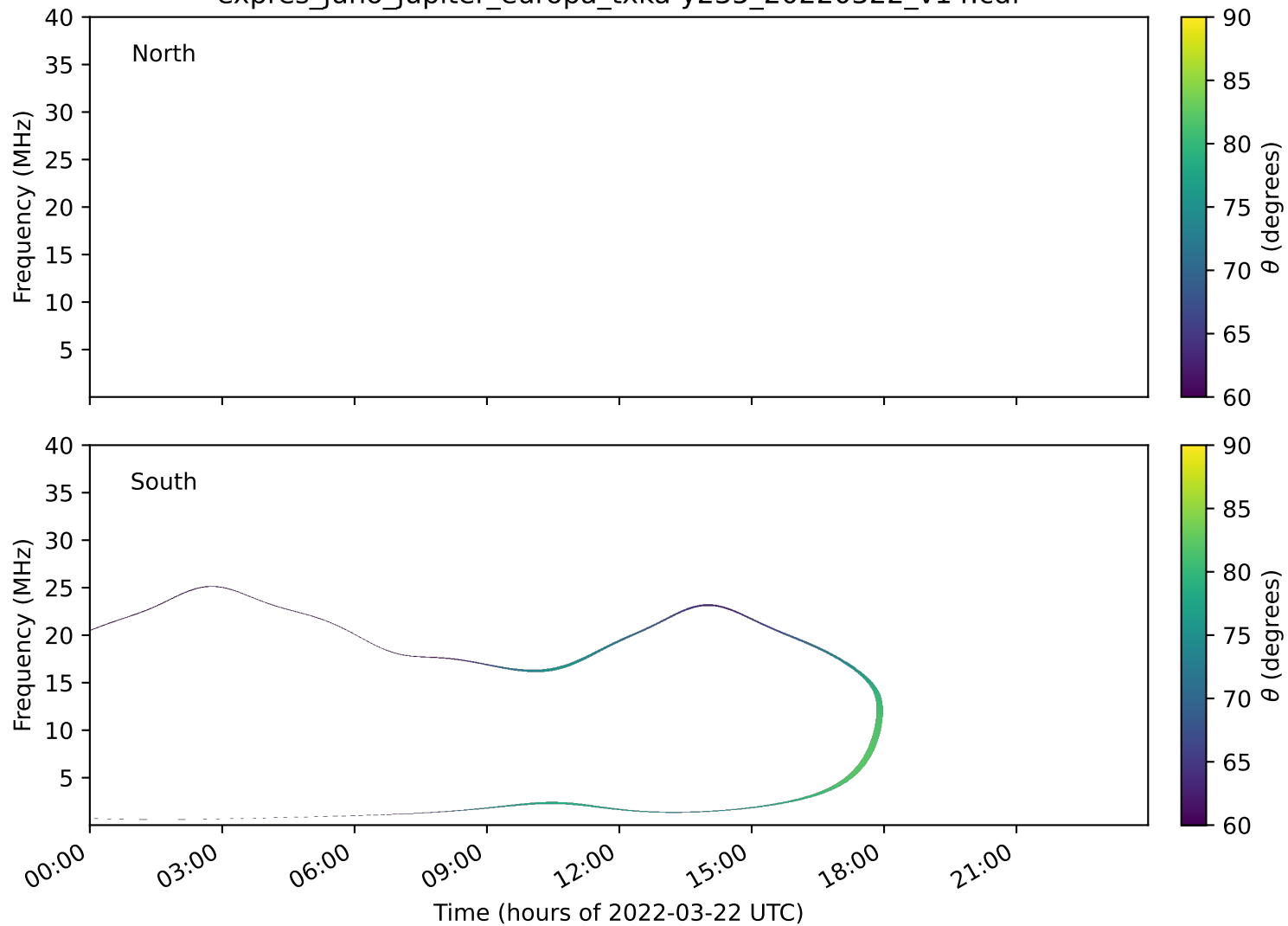
expres_juno_jupiter_europa_txka-y235_20220322_v14.cdf
