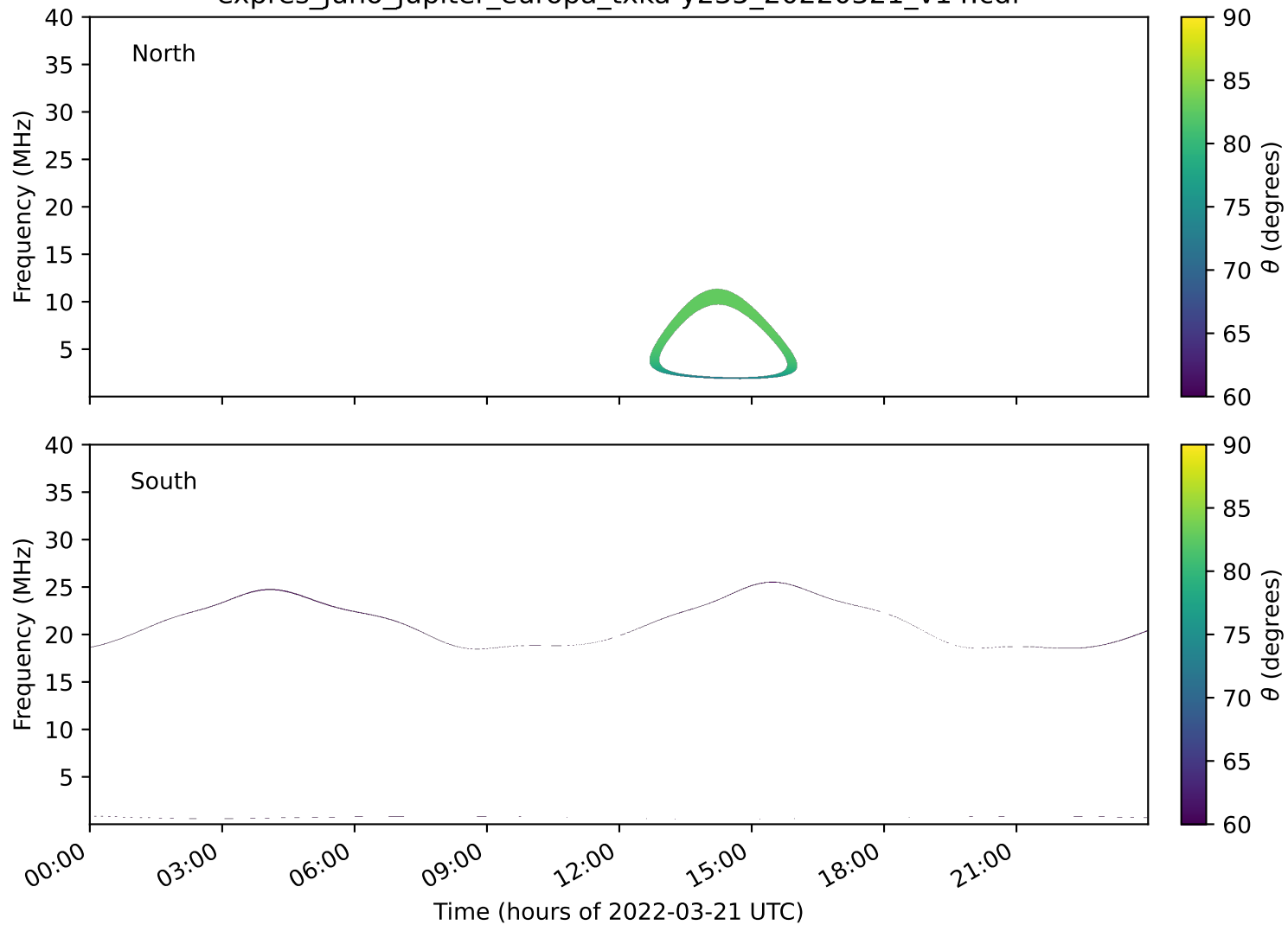
expres_juno_jupiter_europa_txka-y235_20220321_v14.cdf
