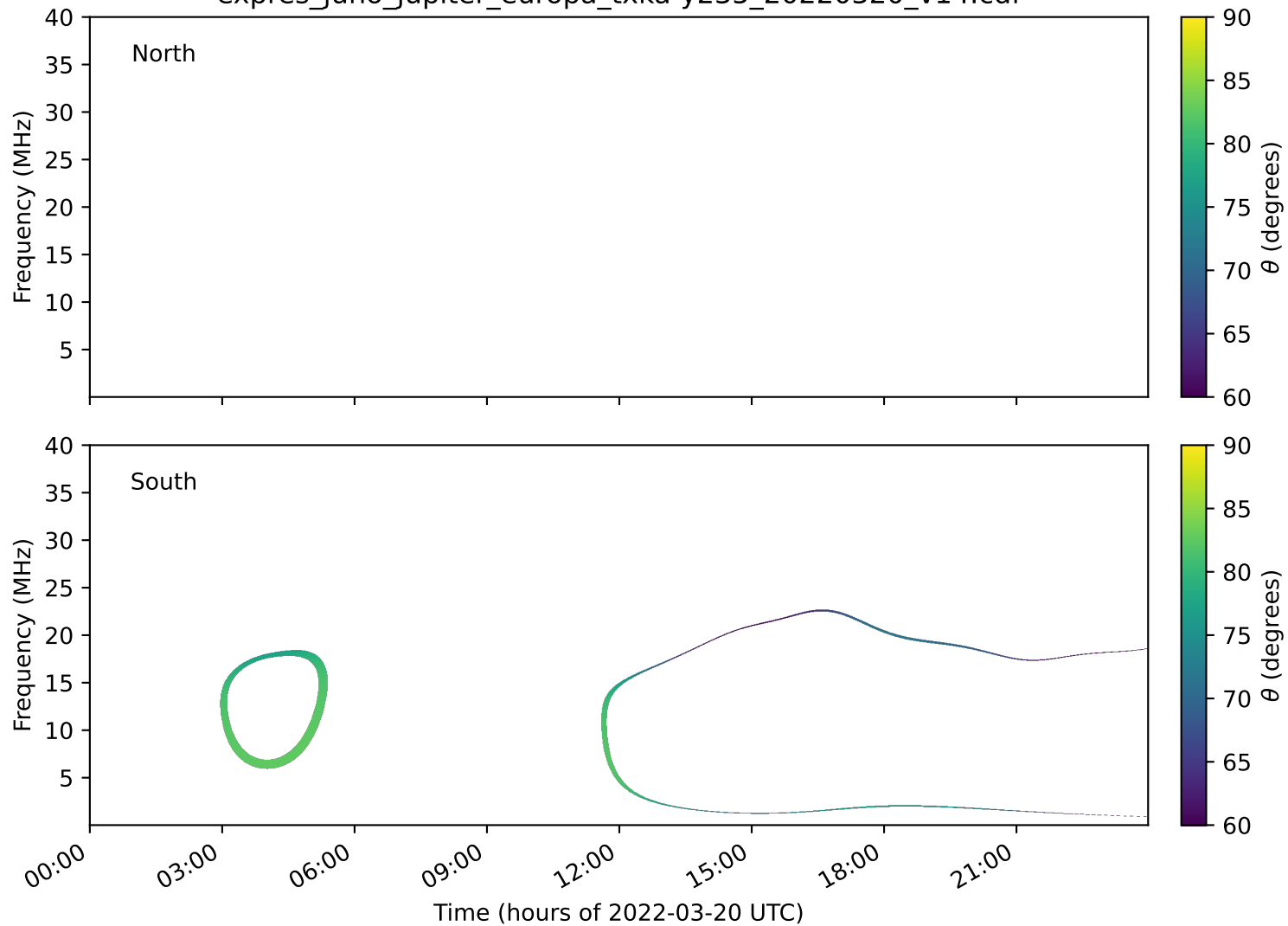
expres_juno_jupiter_europa_txka-y235_20220320_v14.cdf
