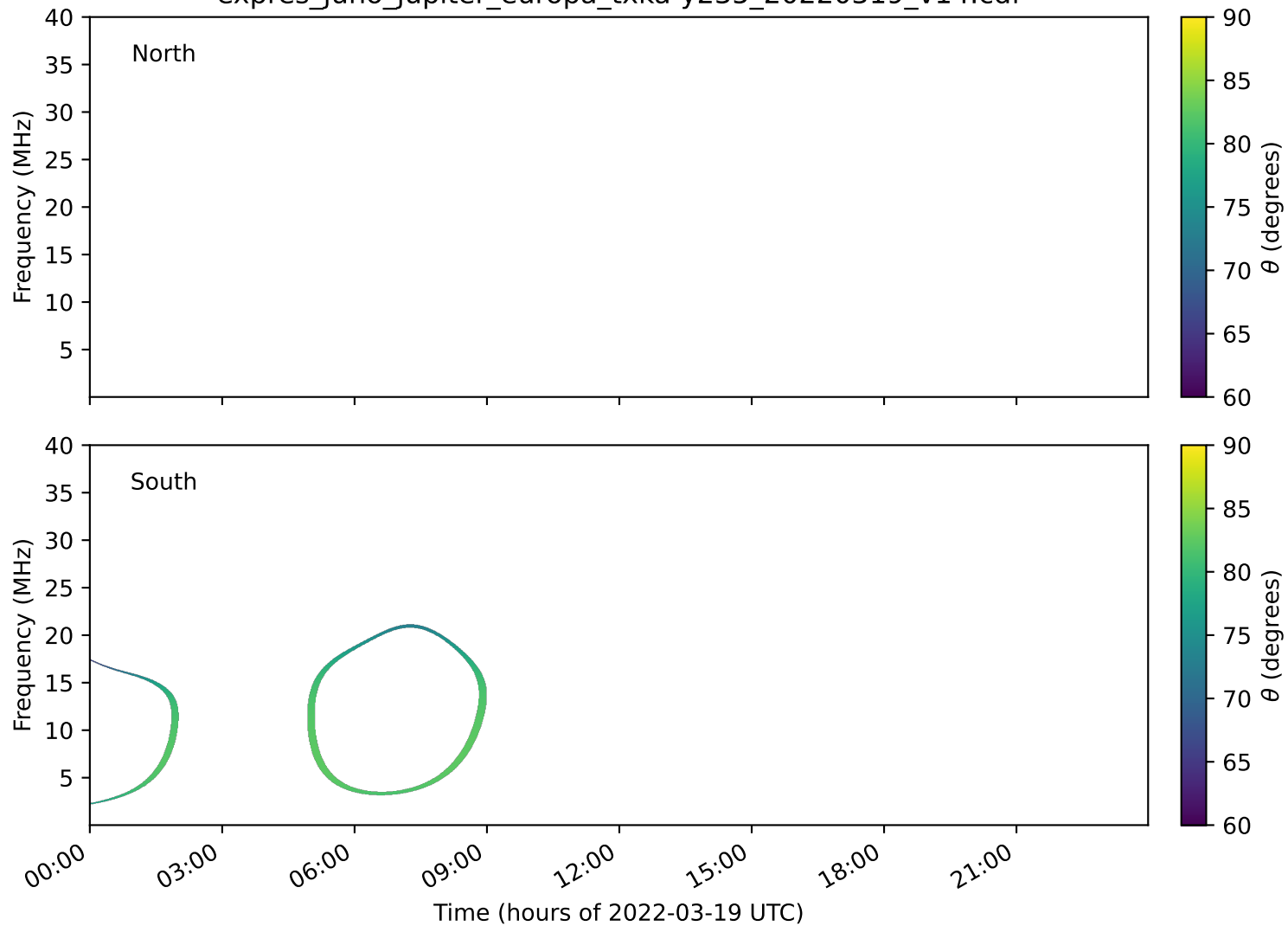
expres_juno_jupiter_europa_txka-y235_20220319_v14.cdf
