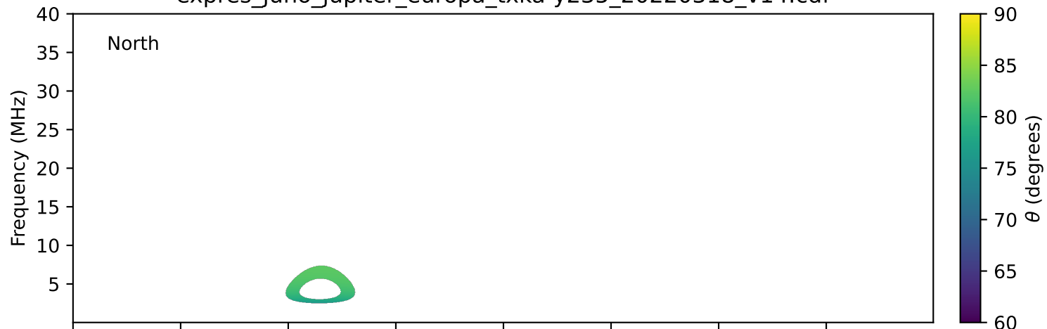
expres_juno_jupiter_europa_txka-y235_20220318_v14.cdf
