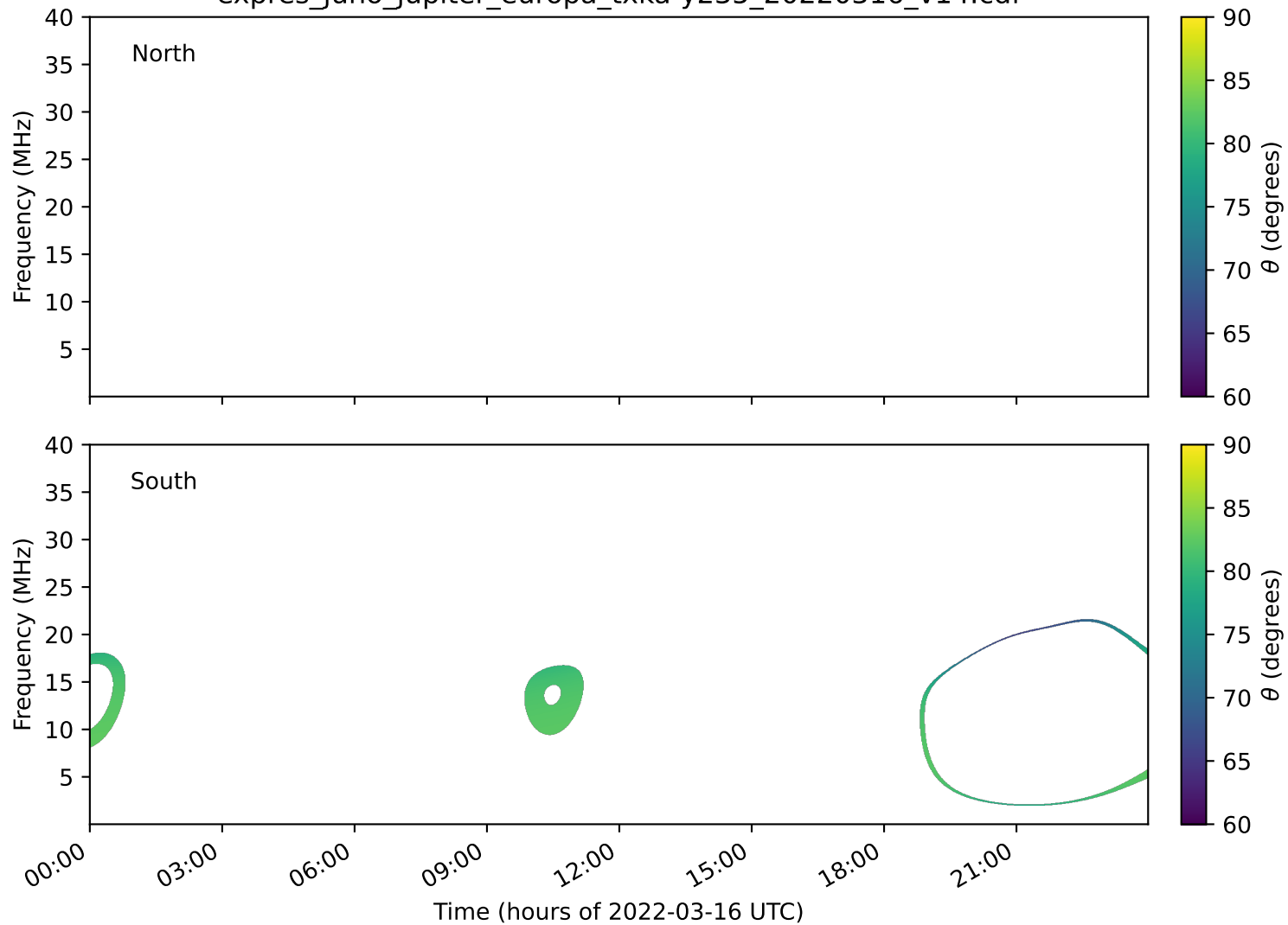
expres_juno_jupiter_europa_txka-y235_20220316_v14.cdf
