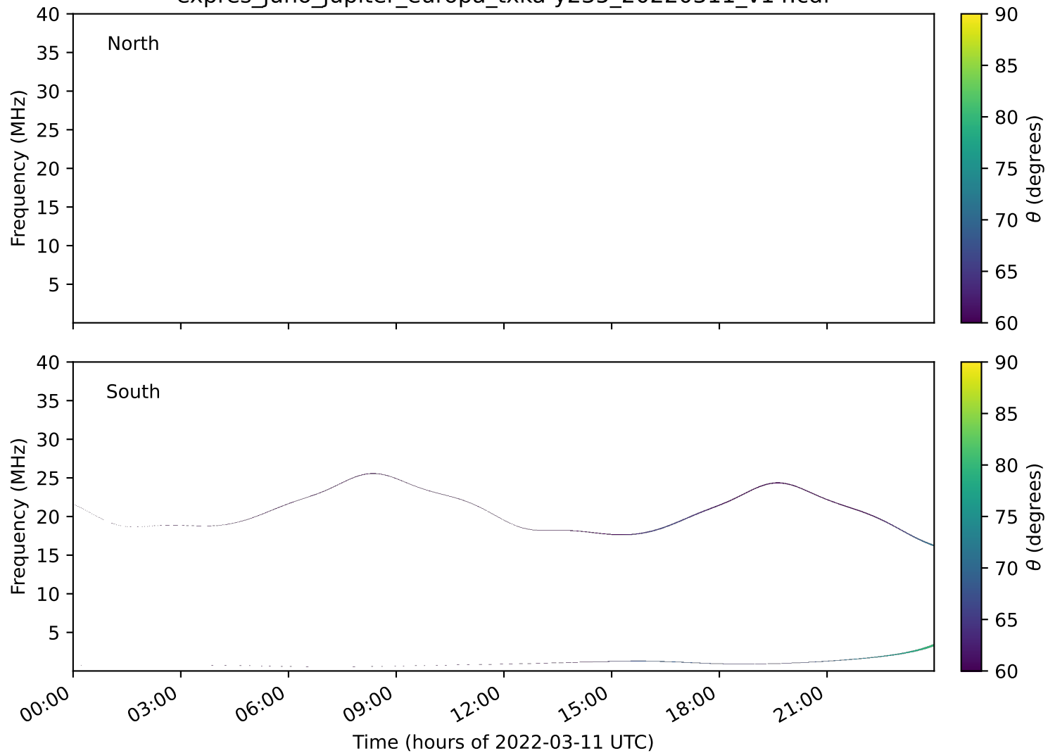
expres_juno_jupiter_europa_txka-y235_20220311_v14.cdf
