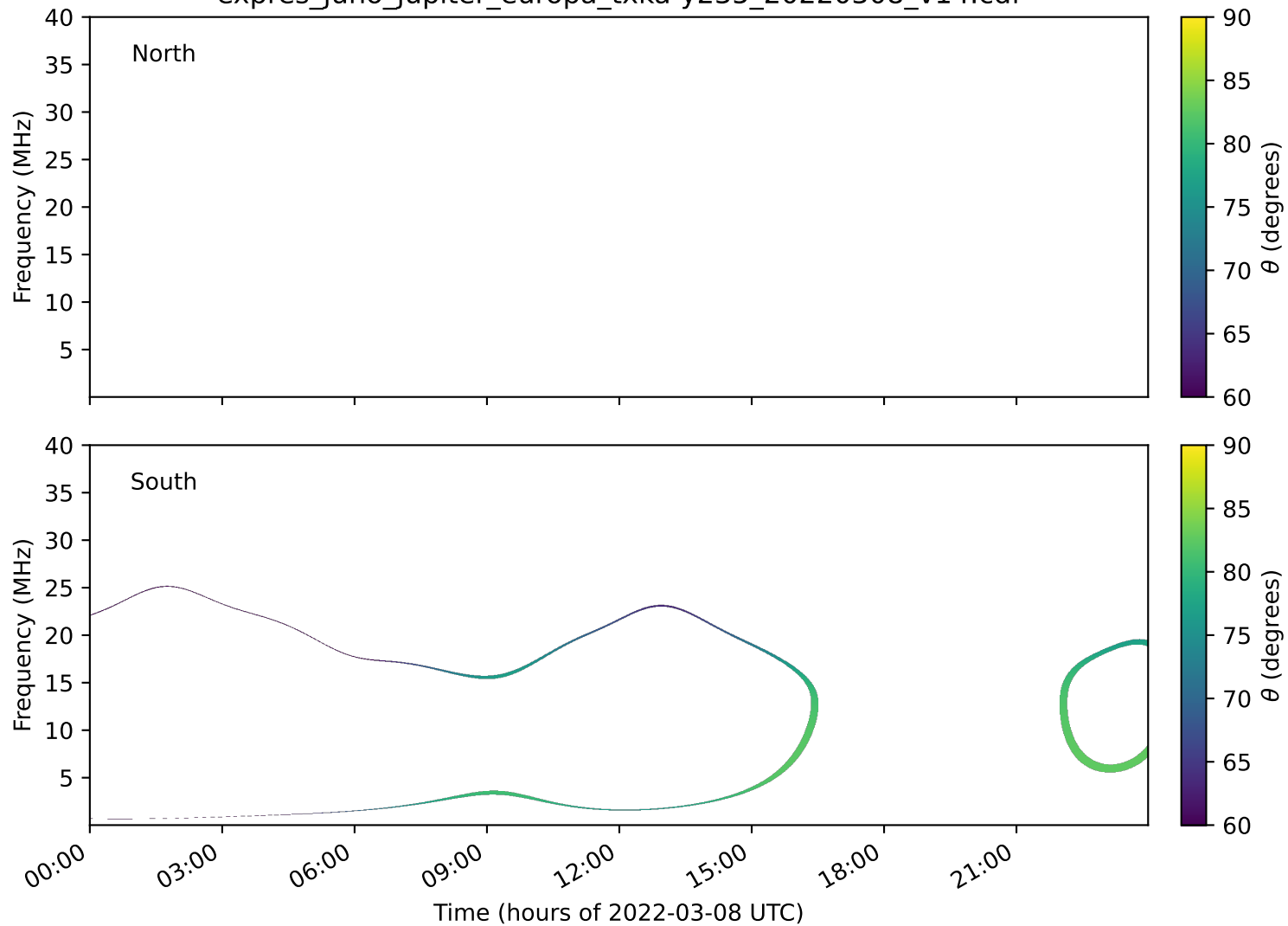
expres_juno_jupiter_europa_txka-y235_20220308_v14.cdf
