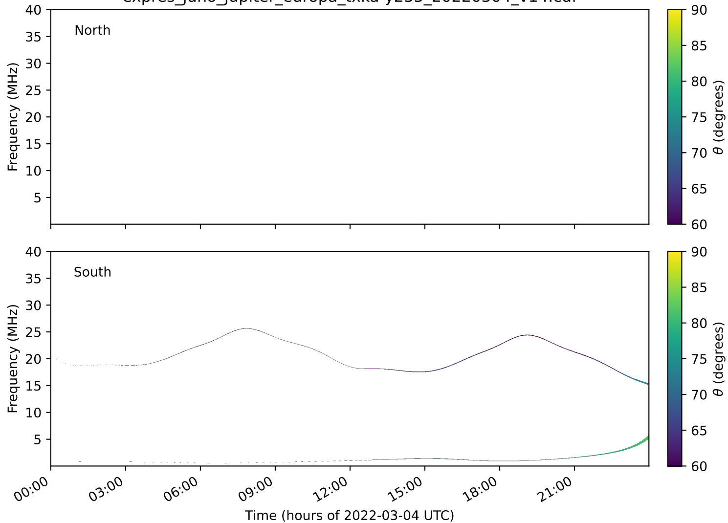
expres_juno_jupiter_europa_txka-y235_20220304_v14.cdf
