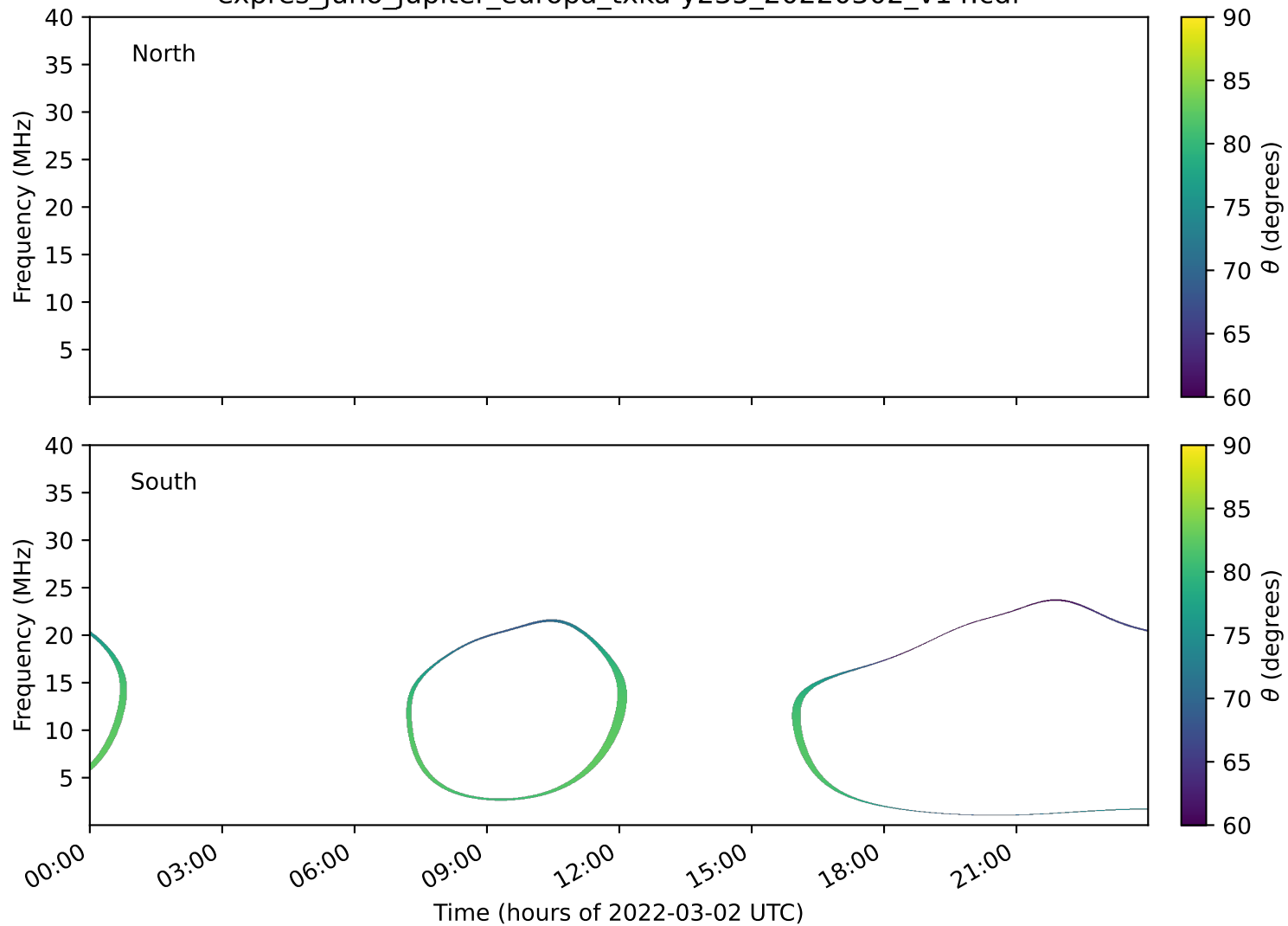
expres_juno_jupiter_europa_txka-y235_20220302_v14.cdf
