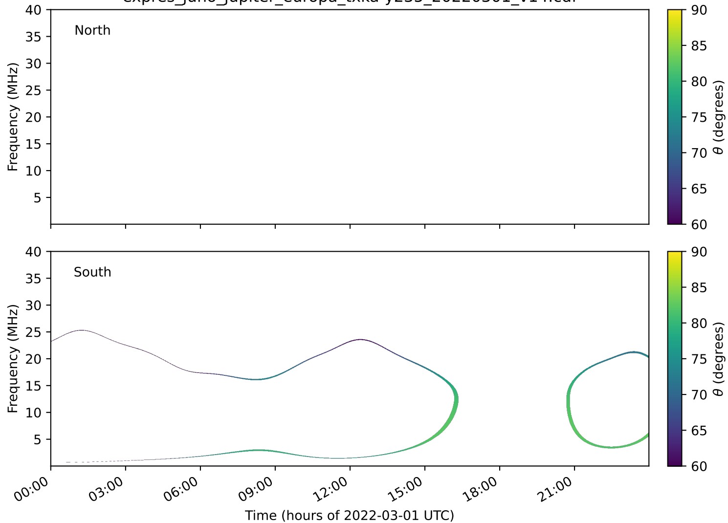
expres_juno_jupiter_europa_txka-y235_20220301_v14.cdf
