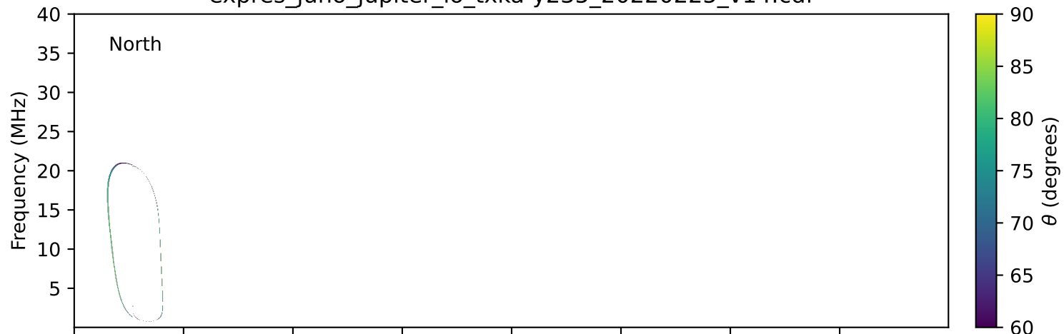
expres_juno_jupiter_io_txka-y235_20220225_v14.cdf
