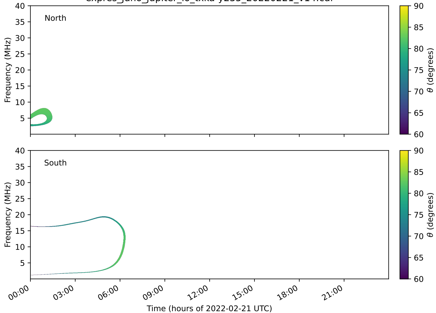
expres_juno_jupiter_io_txka-y235_20220221_v14.cdf
