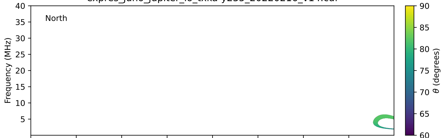
expres_juno_jupiter_io_txka-y235_20220216_v14.cdf
