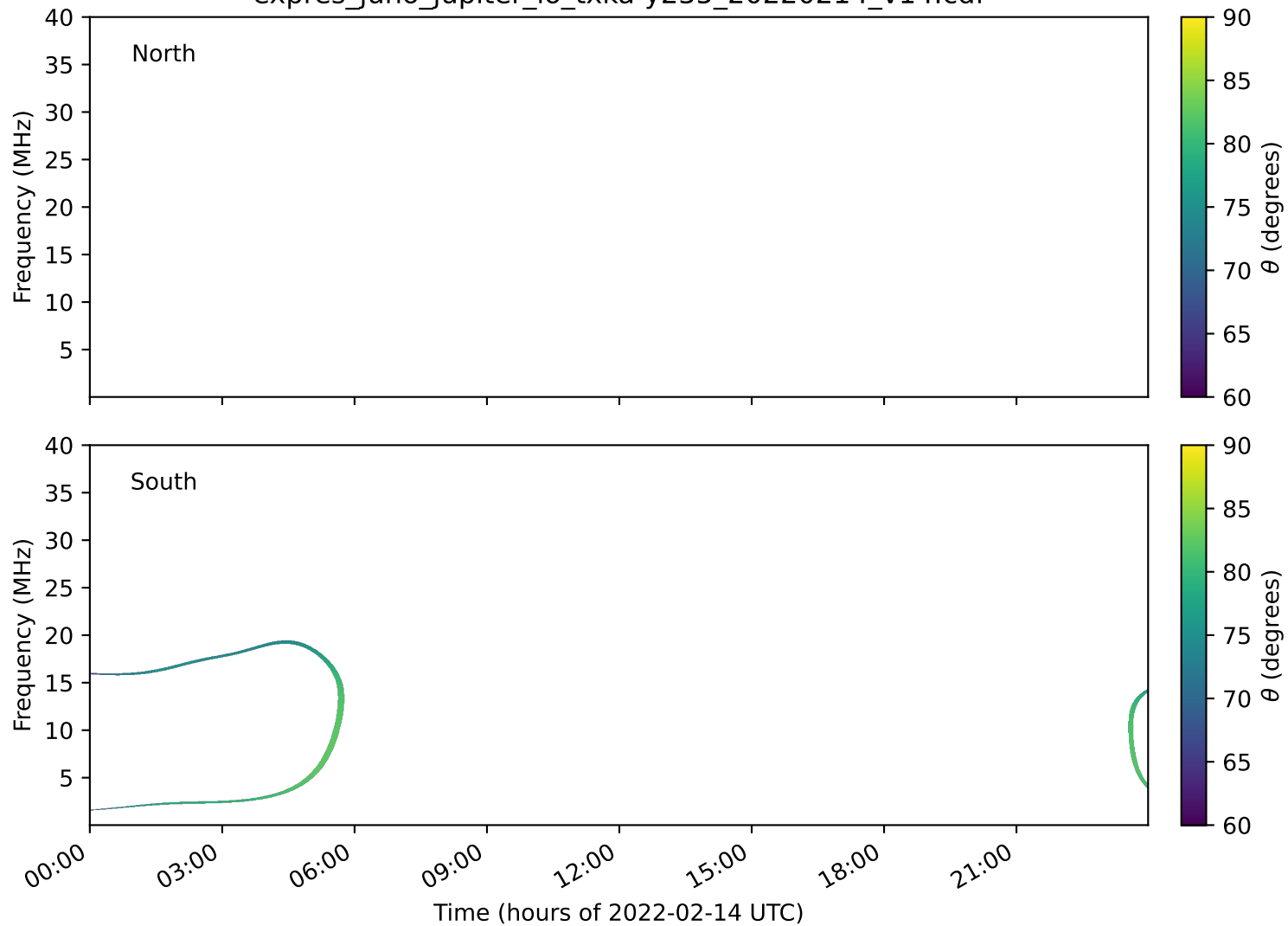
expres_juno_jupiter_io_txka-y235_20220214_v14.cdf
