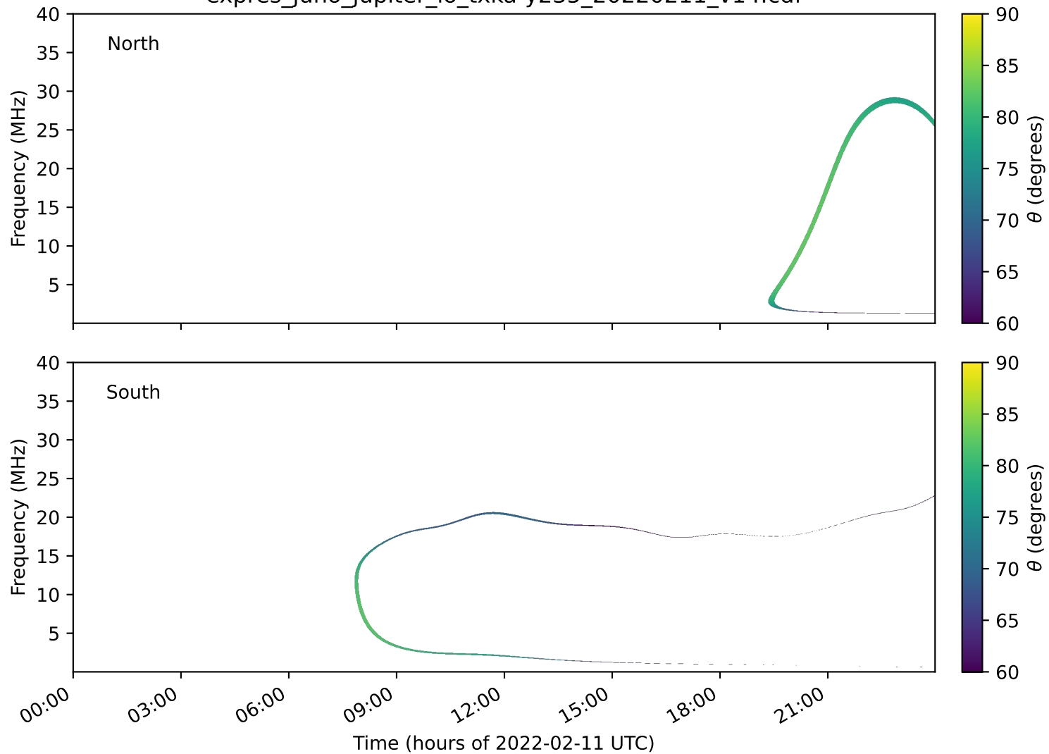
expres_juno_jupiter_io_txka-y235_20220211_v14.cdf
