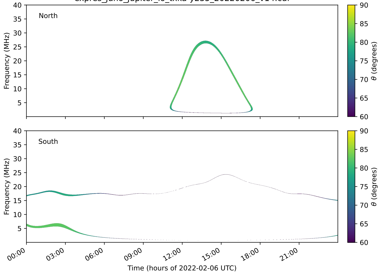
expres_juno_jupiter_io_txka-y235_20220206_v14.cdf
