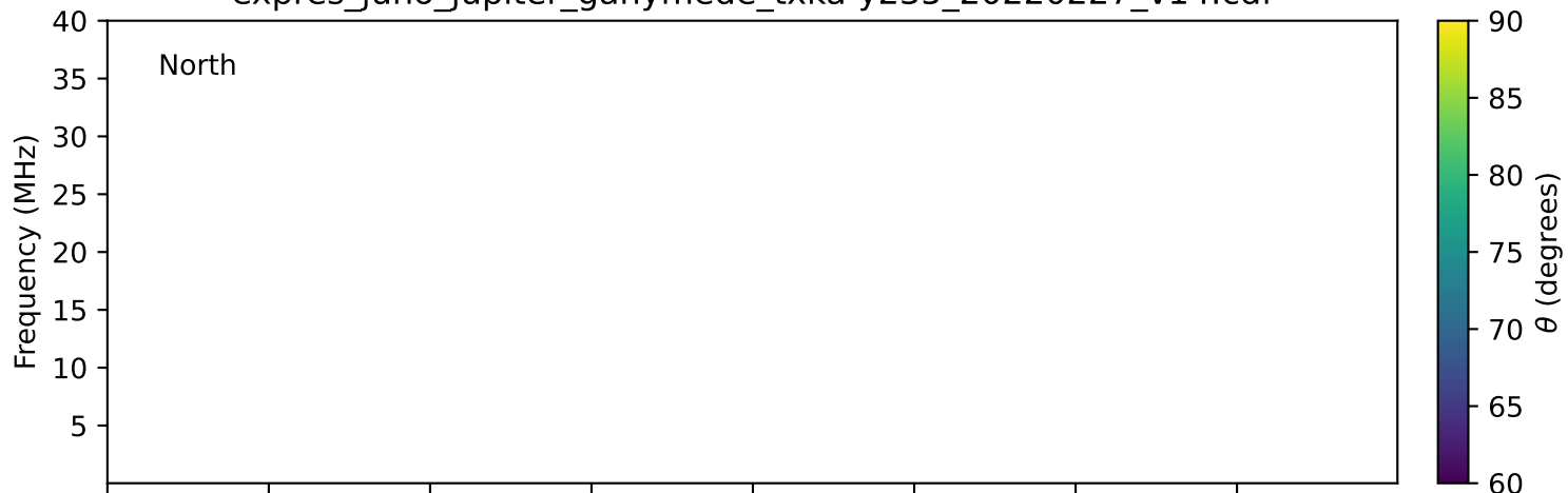
expres_juno_jupiter_ganymede_txka-y235_20220227_v14.cdf
