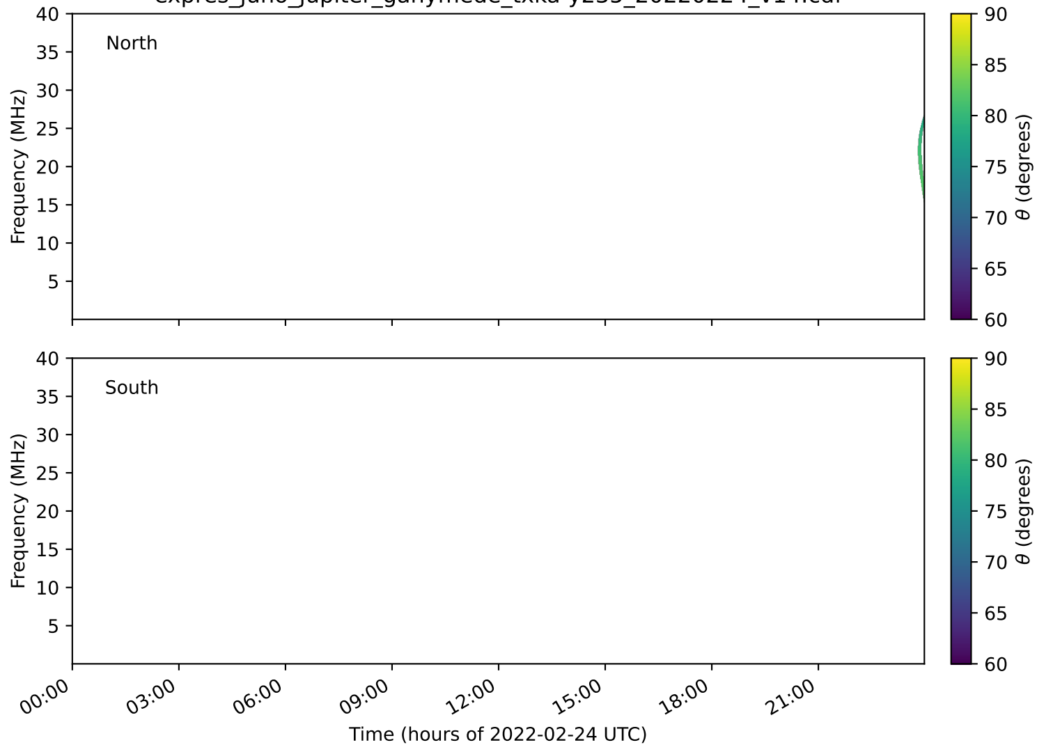
expres_juno_jupiter_ganymede_txka-y235_20220224_v14.cdf
