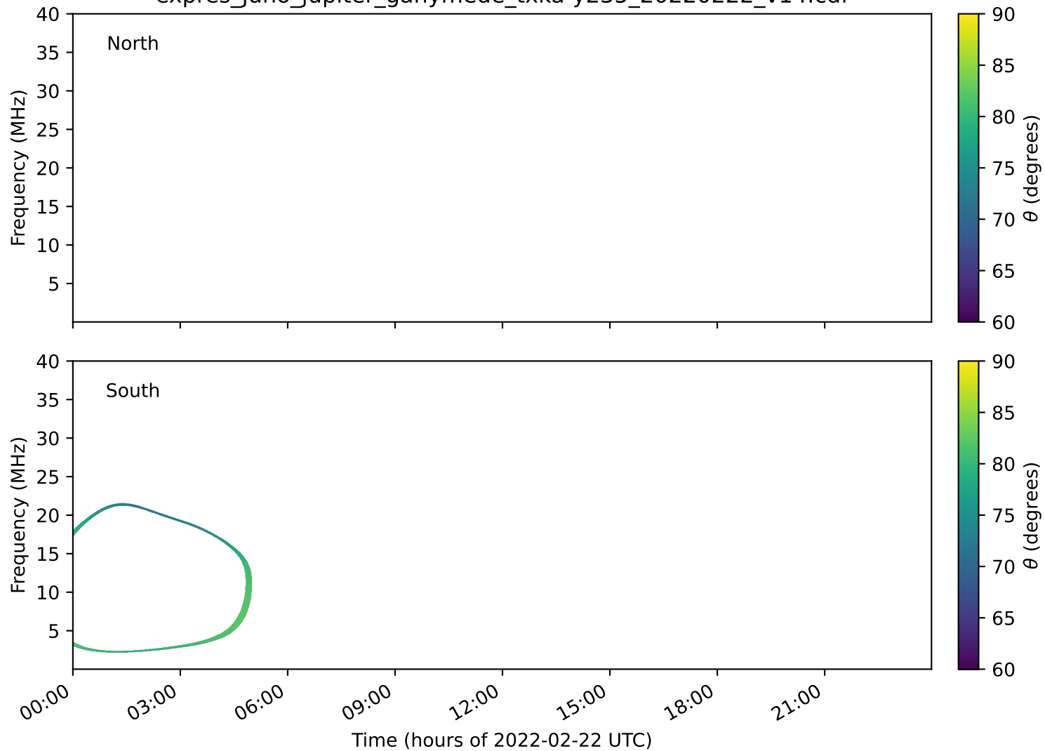
expres_juno_jupiter_ganymede_txka-y235_20220222_v14.cdf
