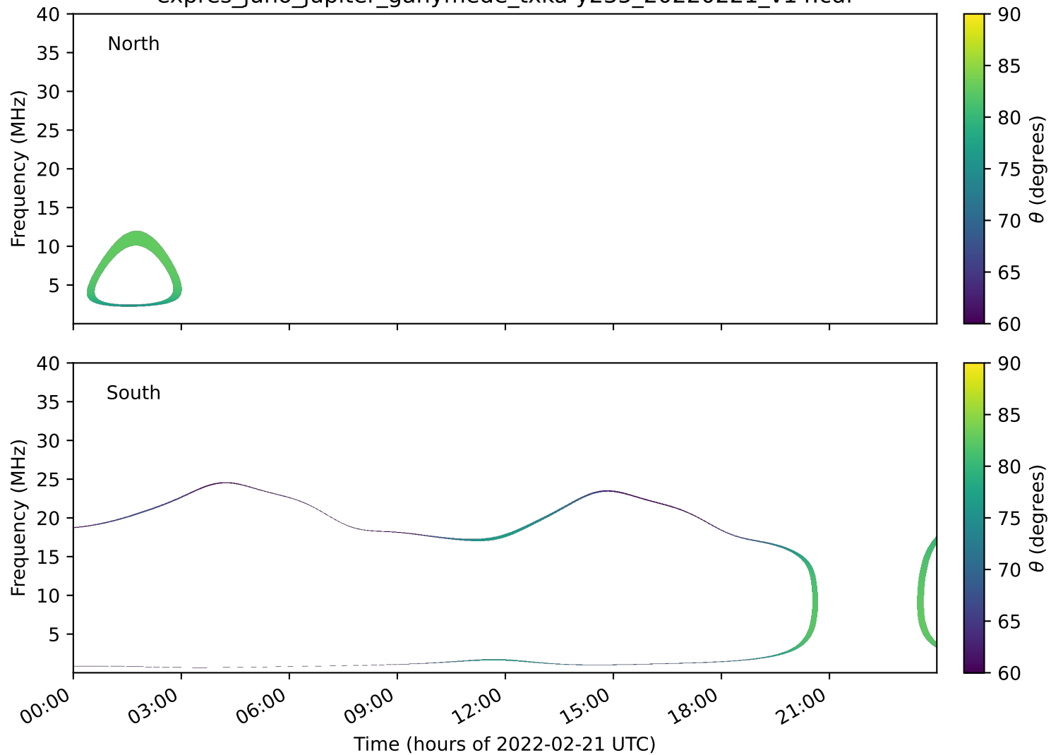
expres_juno_jupiter_ganymede_txka-y235_20220221_v14.cdf
