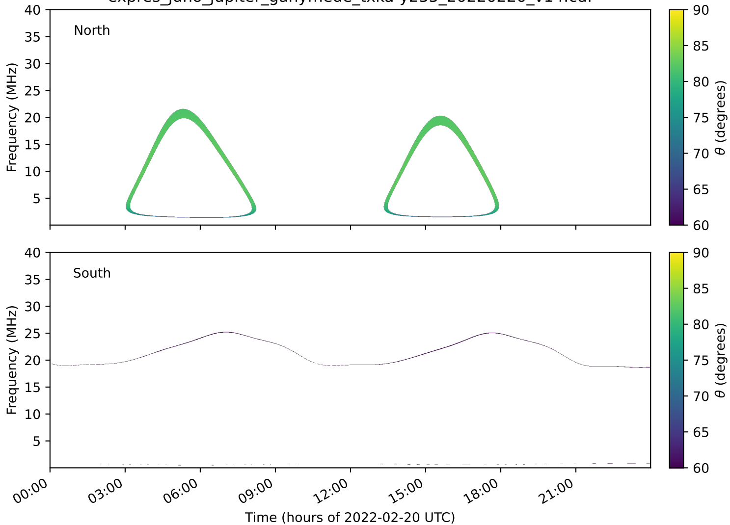
expres_juno_jupiter_ganymede_txka-y235_20220220_v14.cdf
