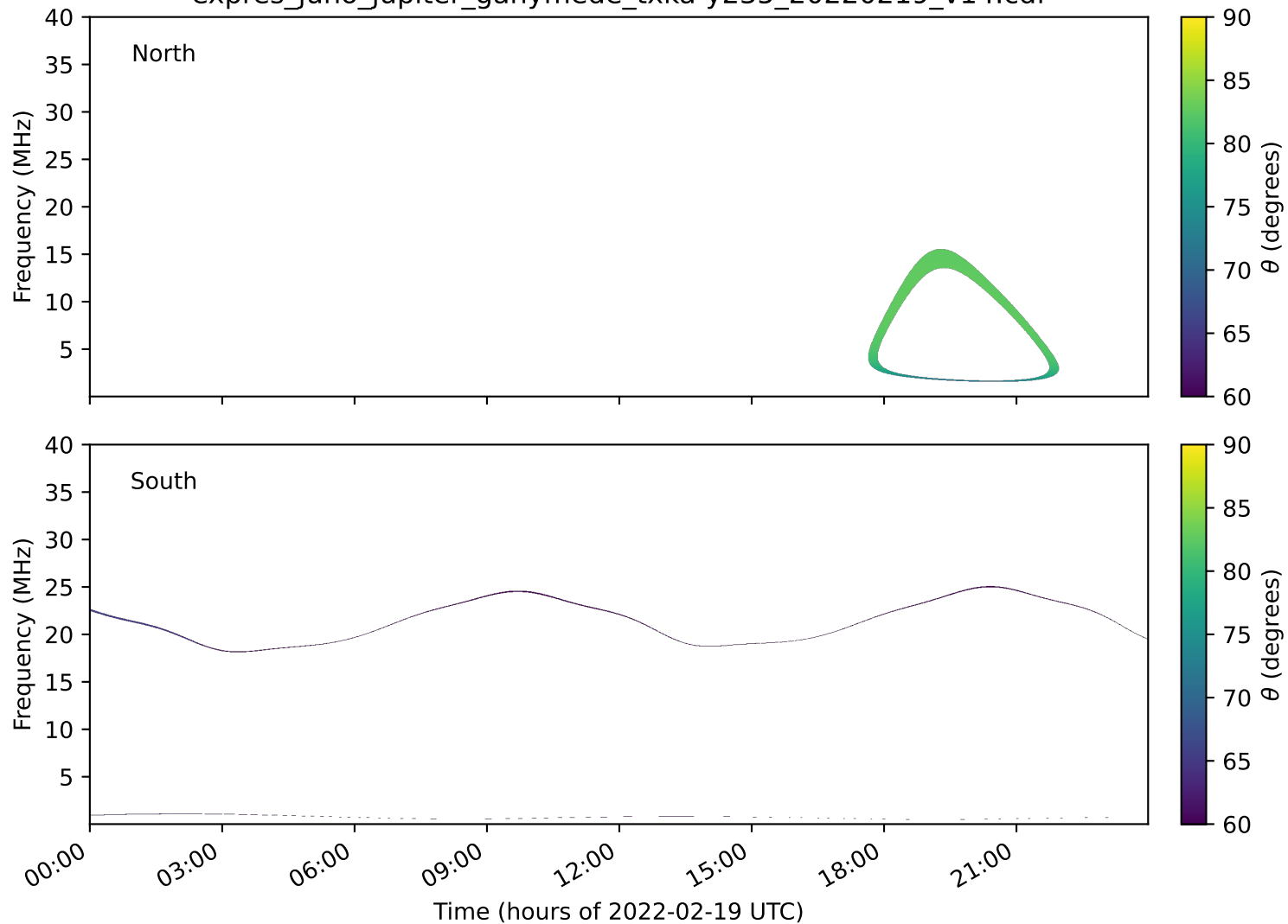
expres_juno_jupiter_ganymede_txka-y235_20220219_v14.cdf
