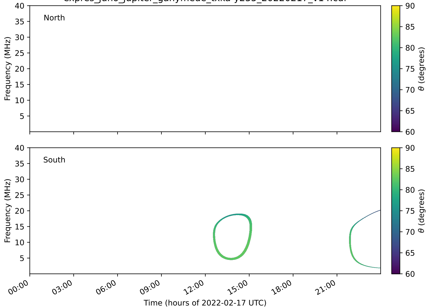
expres_juno_jupiter_ganymede_txka-y235_20220217_v14.cdf
