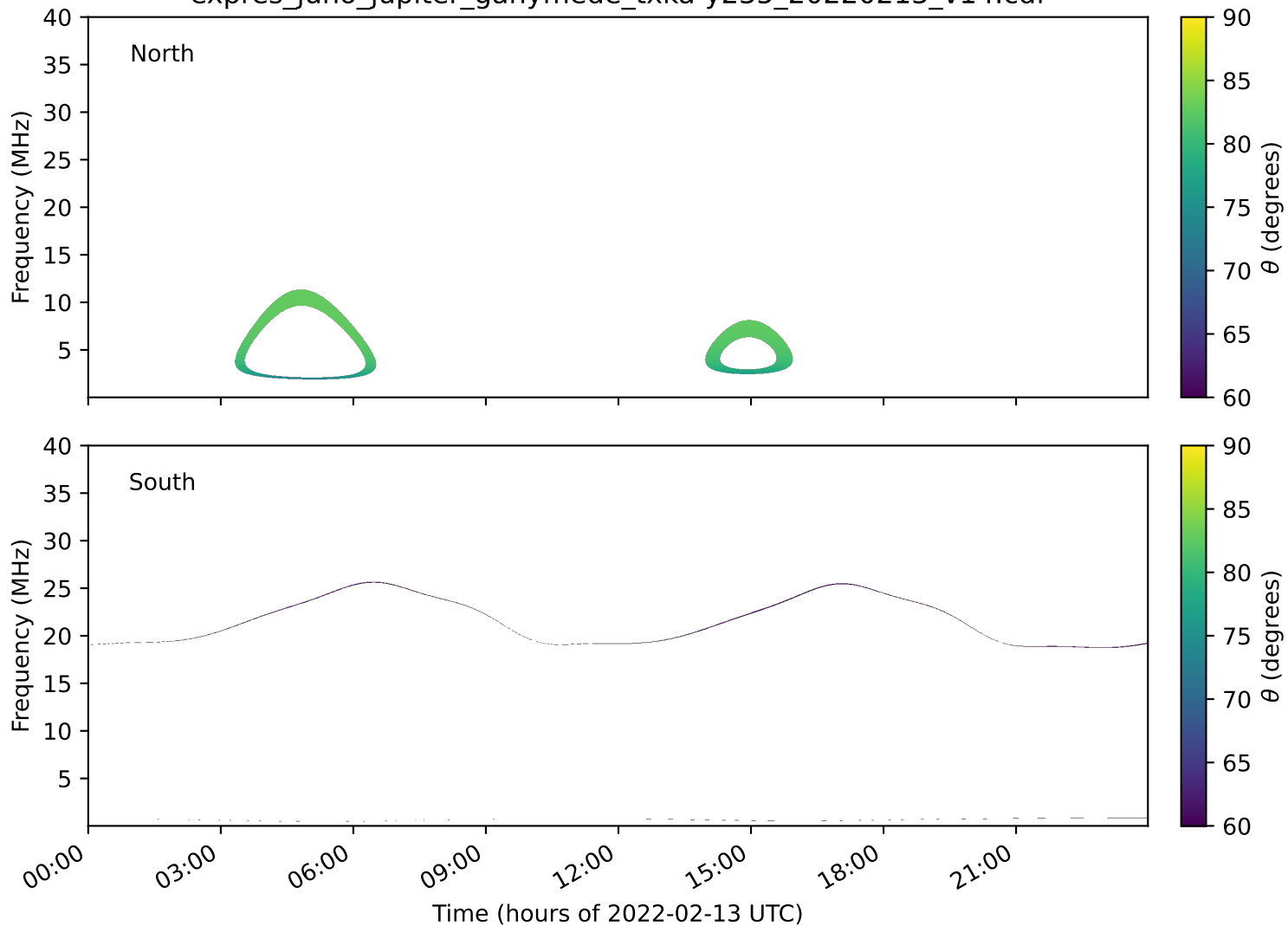
expres_juno_jupiter_ganymede_txka-y235_20220213_v14.cdf
