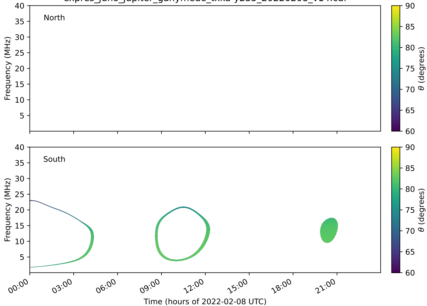
expres_juno_jupiter_ganymede_txka-y235_20220208_v14.cdf
