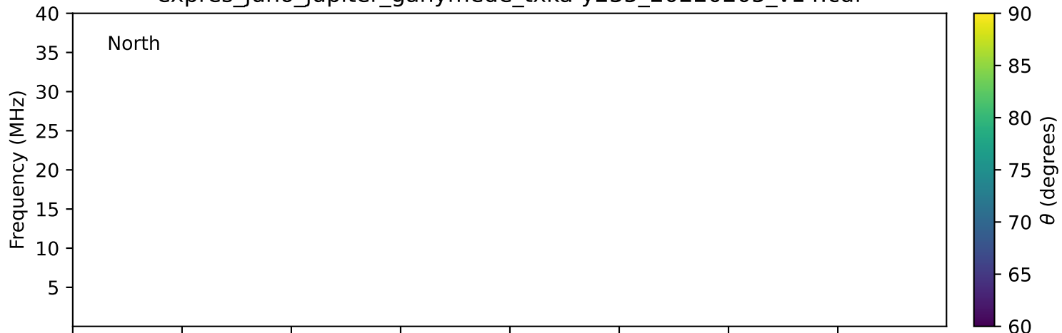
expres_juno_jupiter_ganymede_txka-y235_20220205_v14.cdf
