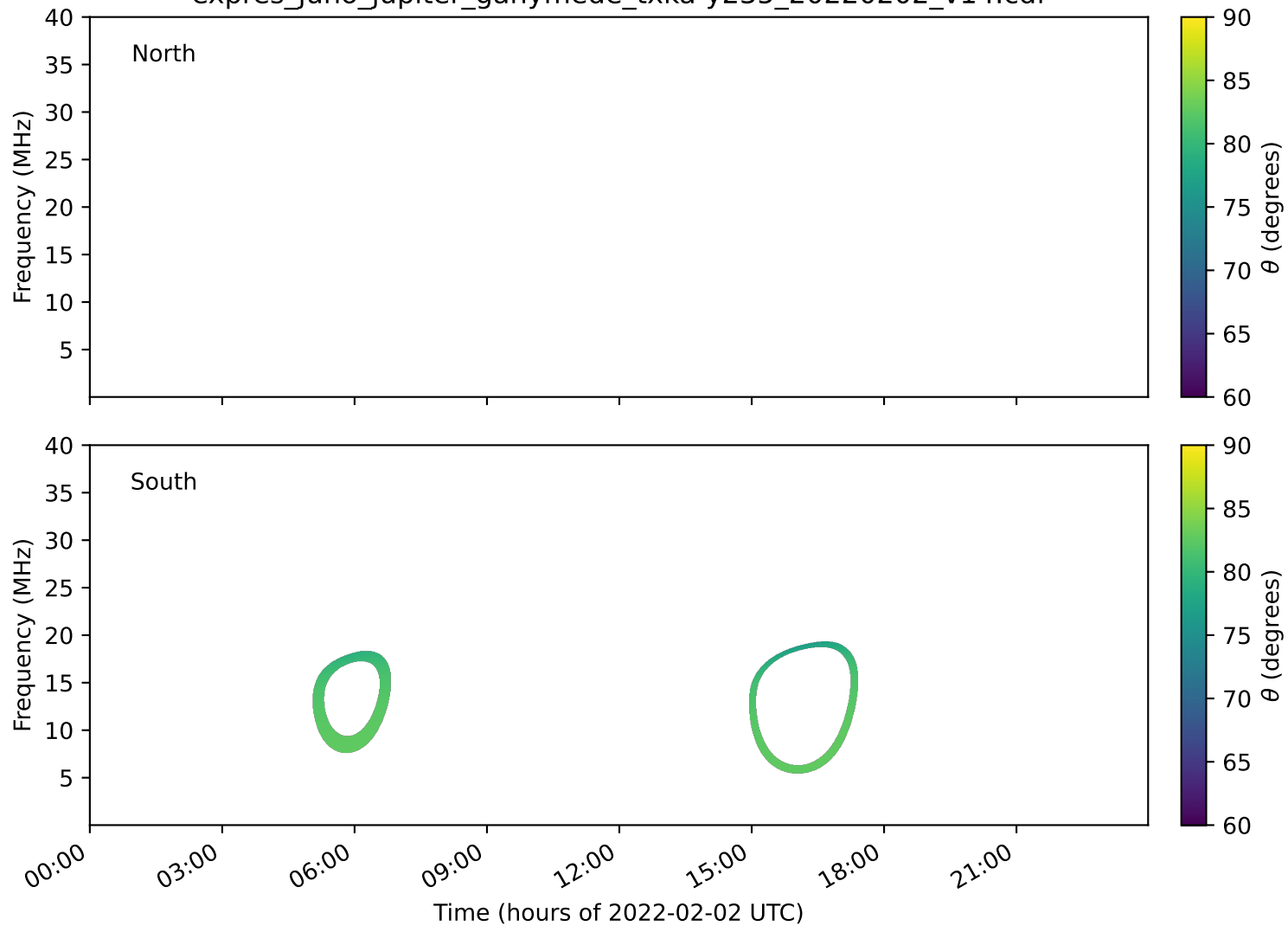
expres_juno_jupiter_ganymede_txka-y235_20220202_v14.cdf
