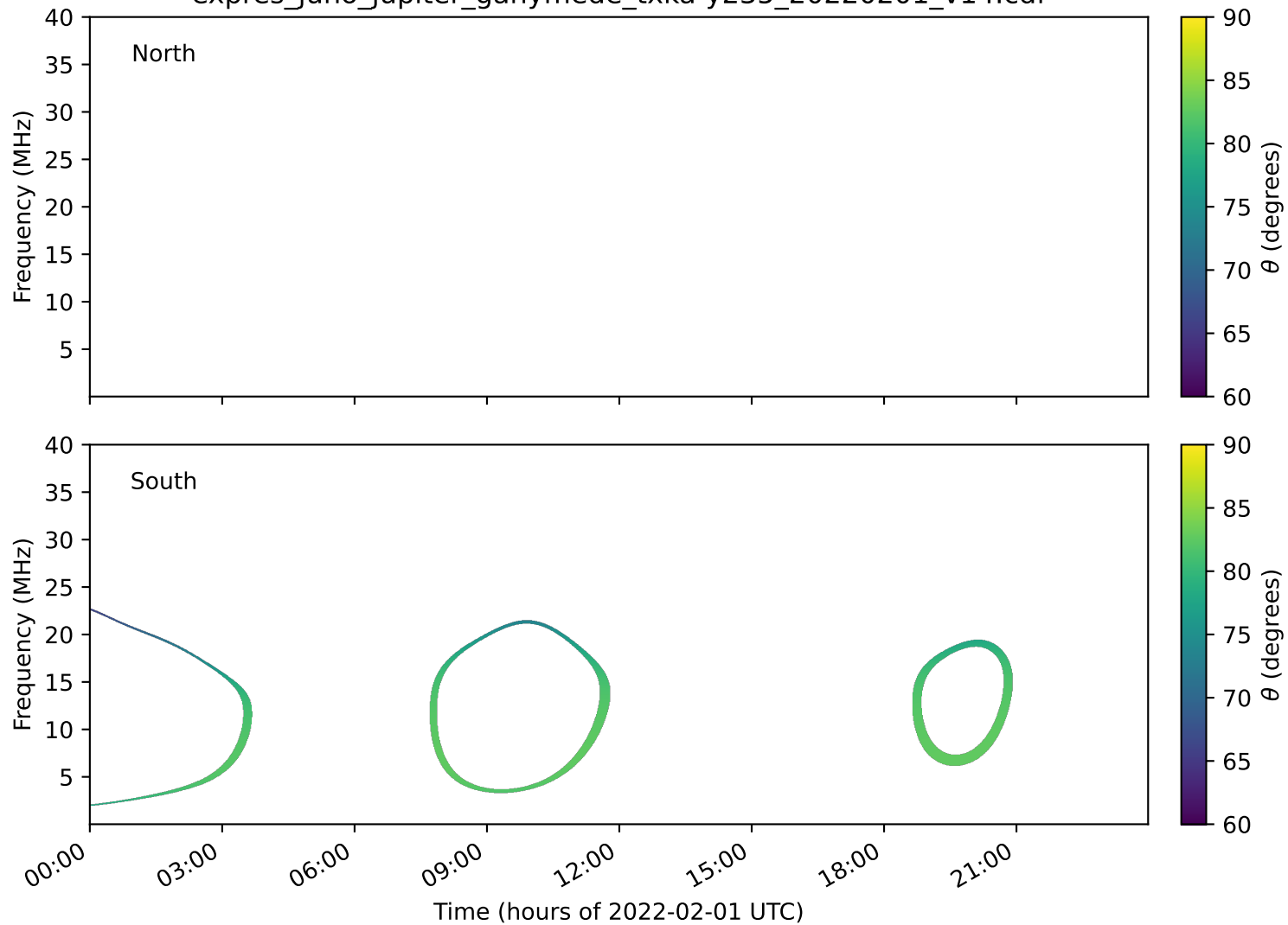
expres_juno_jupiter_ganymede_txka-y235_20220201_v14.cdf
