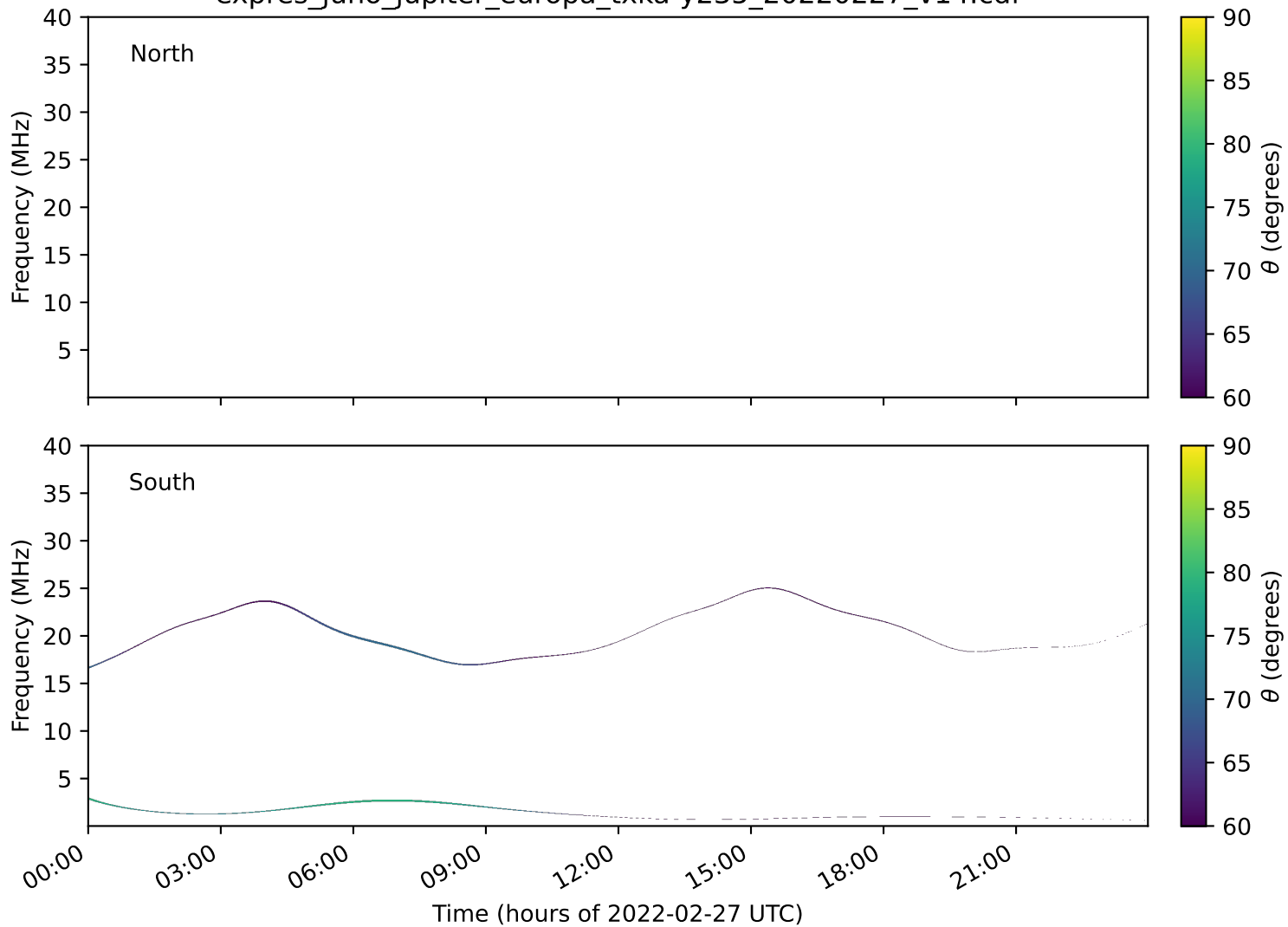
expres_juno_jupiter_europa_txka-y235_20220227_v14.cdf
