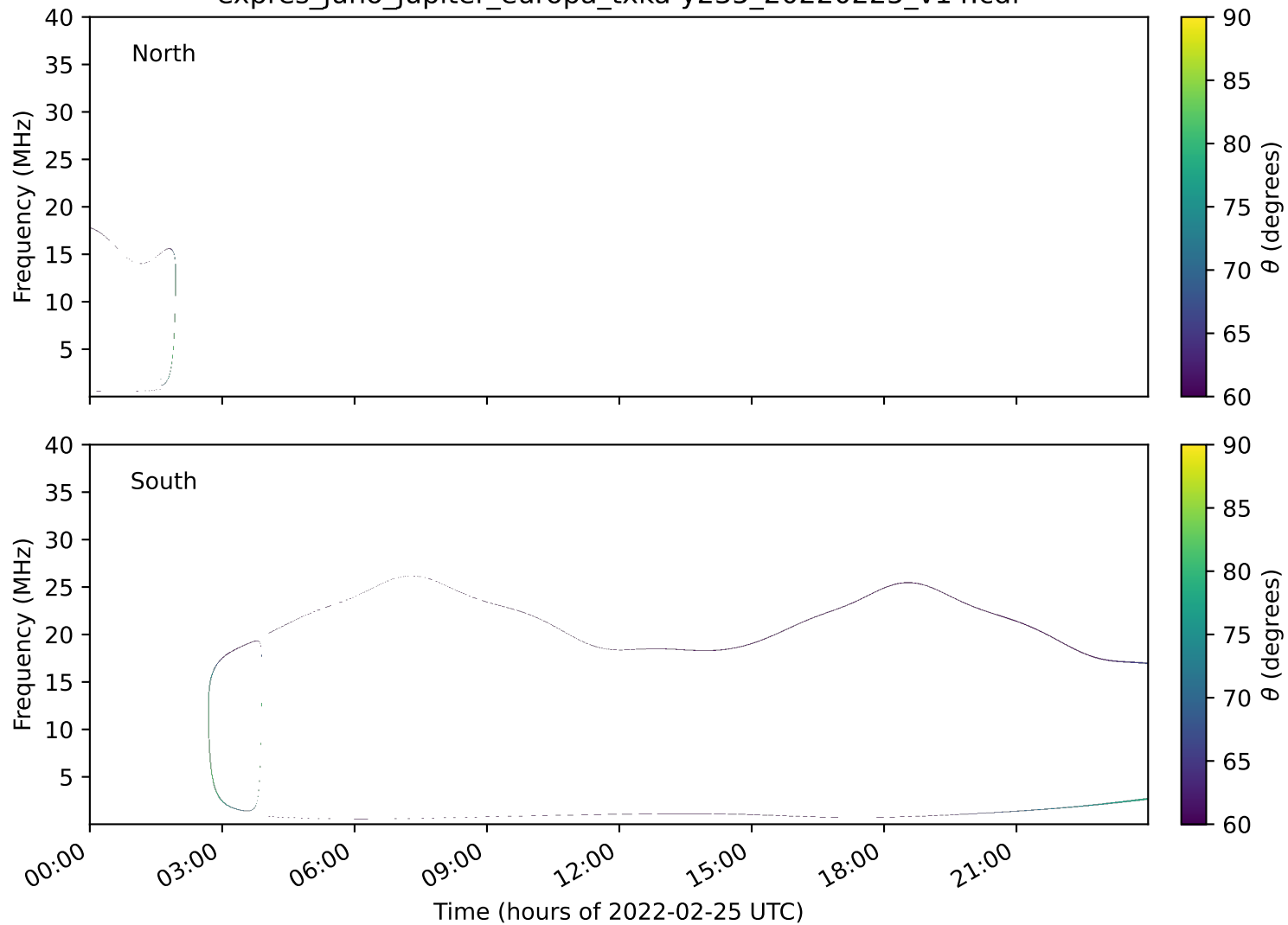
expres_juno_jupiter_europa_txka-y235_20220225_v14.cdf
