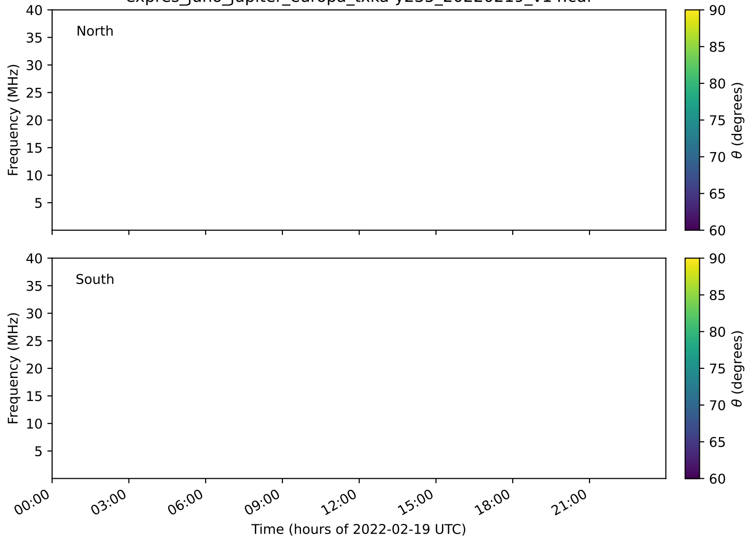
expres_juno_jupiter_europa_txka-y235_20220219_v14.cdf
