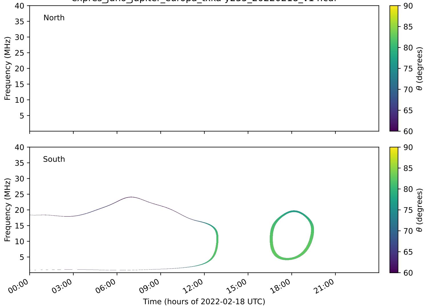
expres_juno_jupiter_europa_txka-y235_20220218_v14.cdf
