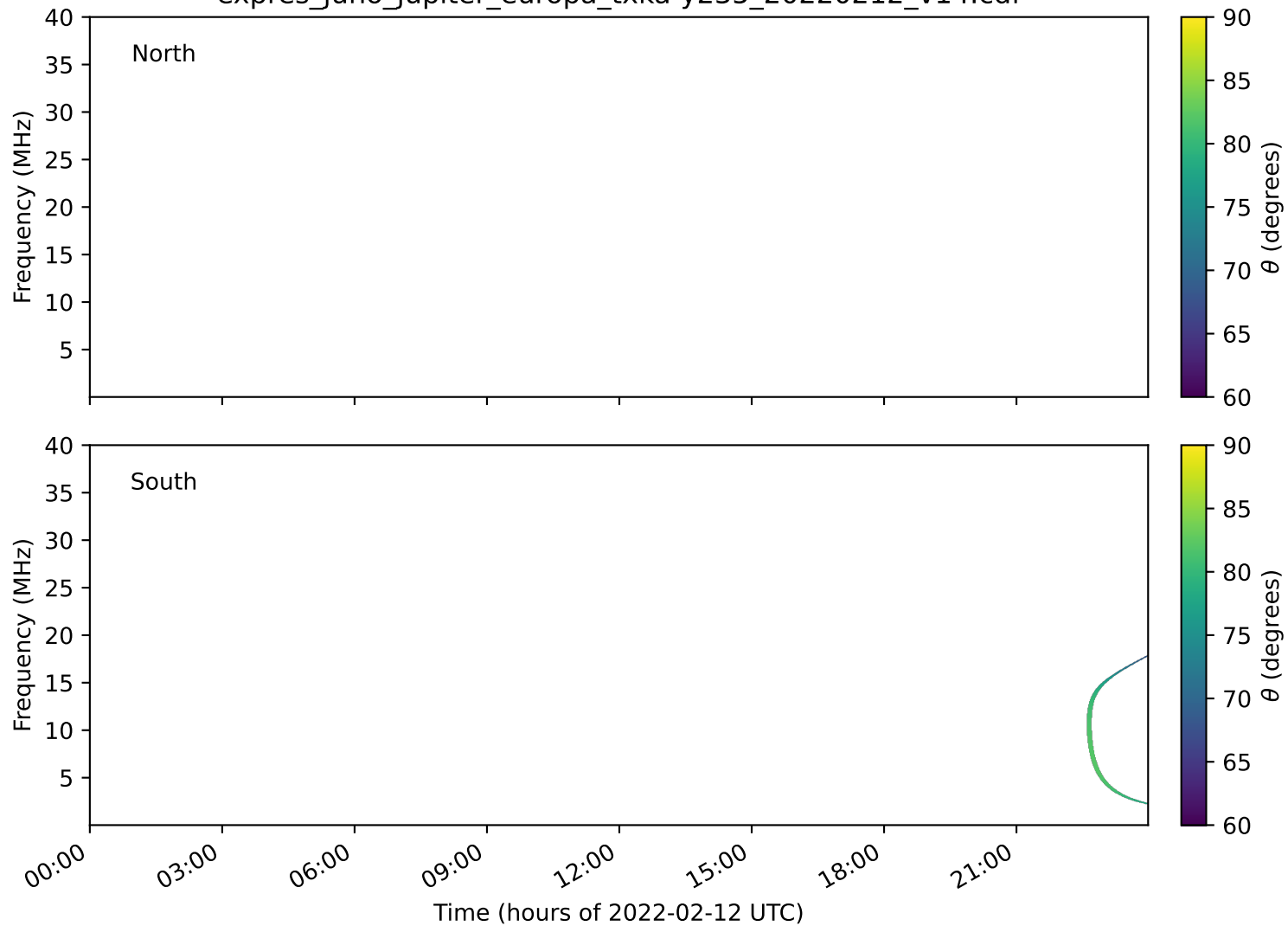
expres_juno_jupiter_europa_txka-y235_20220212_v14.cdf
