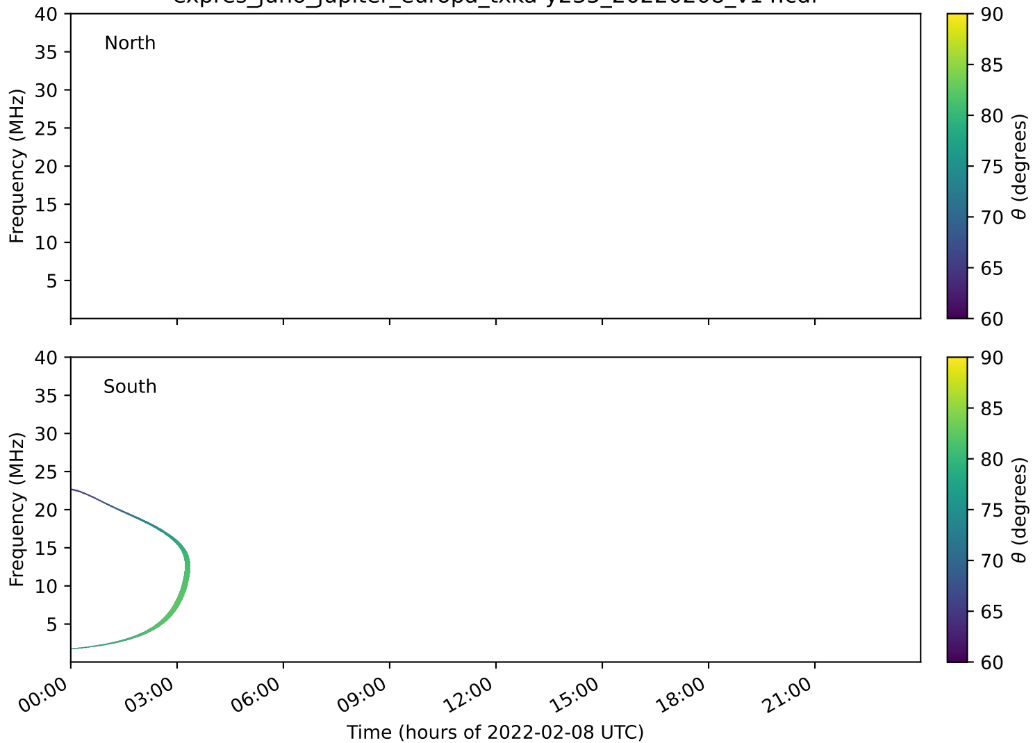
expres_juno_jupiter_europa_txka-y235_20220208_v14.cdf
