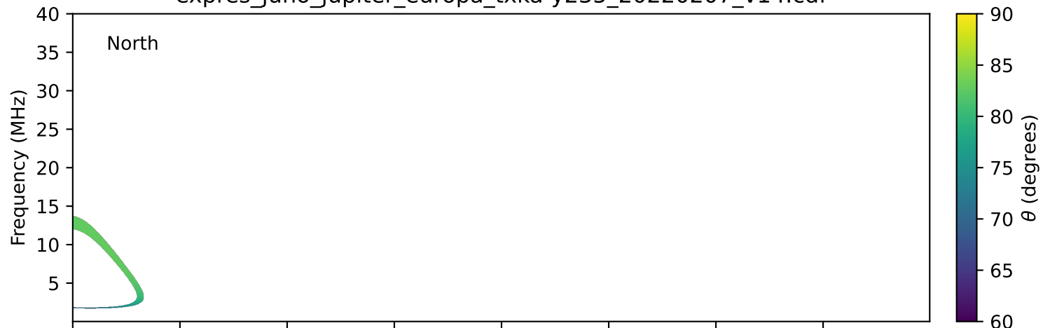
expres_juno_jupiter_europa_txka-y235_20220207_v14.cdf
