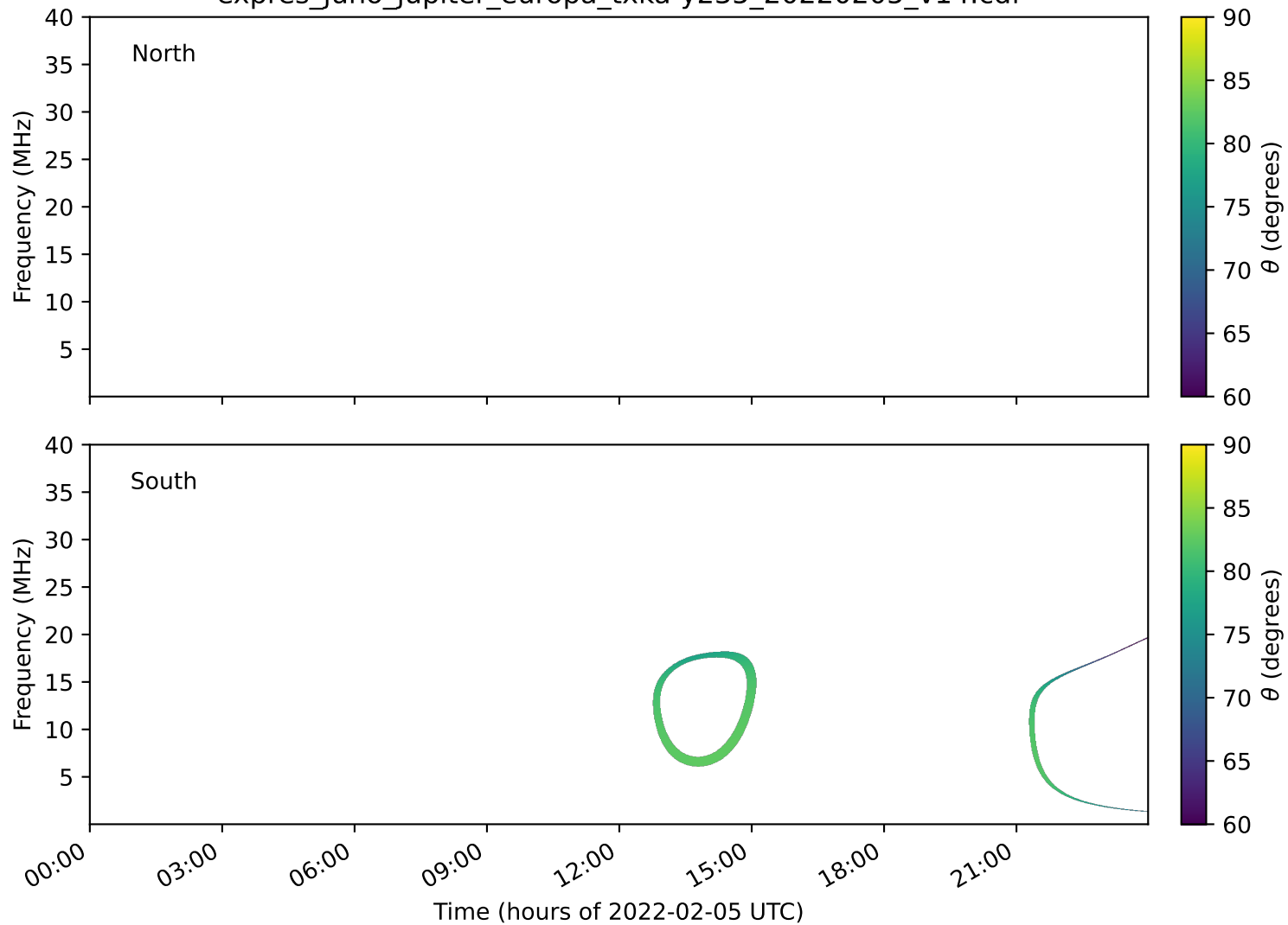
expres_juno_jupiter_europa_txka-y235_20220205_v14.cdf
