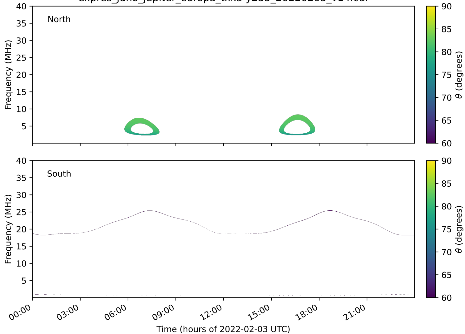
expres_juno_jupiter_europa_txka-y235_20220203_v14.cdf
