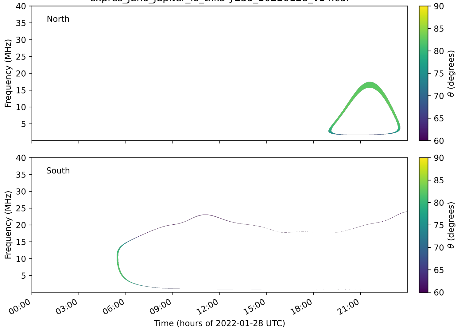
expres_juno_jupiter_io_txka-y235_20220128_v14.cdf
